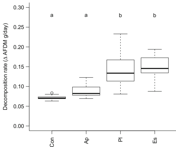
Fig. 1 Processing of leaf litter quantified from measurements of decomposition rates (g loss of AFDM per day). Abbreviations on x-axes: Con, control; Ap, native crayfish ( Austropotamobius pallipes ); Pl, invasive alien crayfish ( Pacifastacus leniusculus ); Es, invasive alien crab ( Eriocheir sinensis ). Letters above boxplots indicate groupings based on post hoc tests
