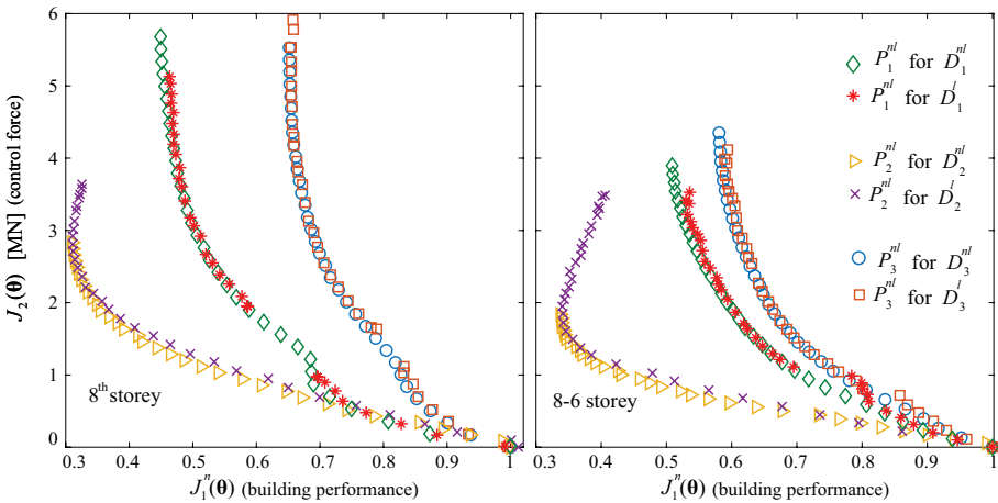
Fig. 12 Performance assessment for the nonlinear structure and for design seismic intensity ( s_c = 1 ) for the drift-sensitive ( O_1 ), acceleration-sensitive ( O_2 ) and balanced ( O_3 ) consequence quantifications. Optimal Pareto fronts are compared to the performance achieved using linear assumption of the structural behavior. Results are presented for 8th storey (left) and 8–6 storey (right) placement. Normalization of J_1 is established with respect to the uncontrolled structure performance for s_c = 1 , for each of the different consequence quantifications
