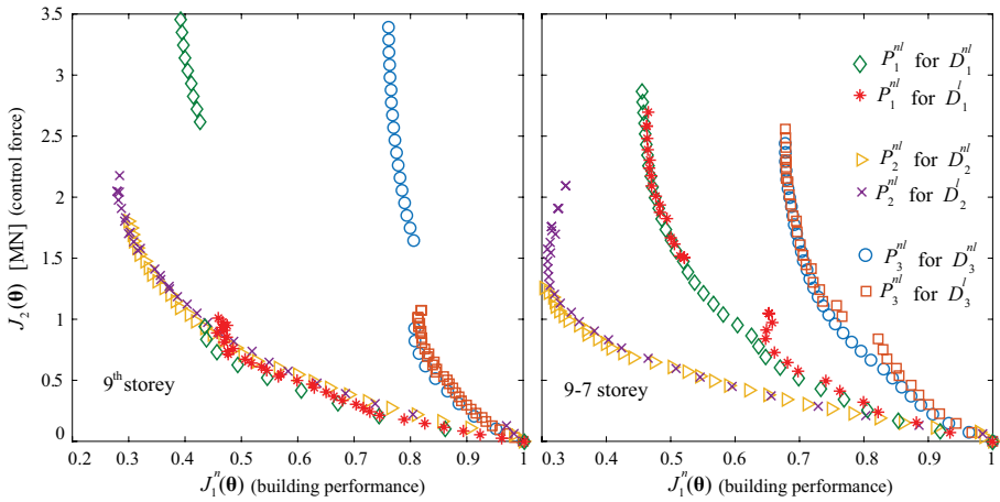
Fig. 11 Performance assessment for the nonlinear structure and for design seismic intensity ( s_c = 1 ) for the drift-sensitive ( O_1 ), acceleration-sensitive ( O_2 ) and balanced ( O_3 ) consequence quantifications. Optimal Pareto fronts are compared to the performance achieved using linear assumption of the structural behavior. Results are presented for 9th storey (left) and 9–7 storey (right) placement. Normalization of J_1 is established with respect to the uncontrolled structure performance for s_c = 1 , for each of the different consequence quantifications
