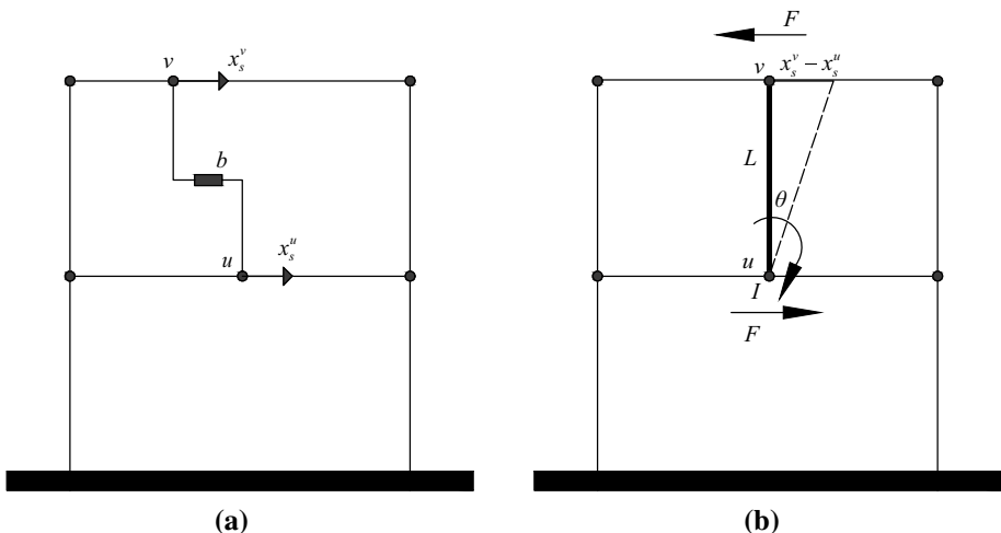
Fig. 15 Modeling of inerter in a finite element program utilizing an isolated rigid bar
