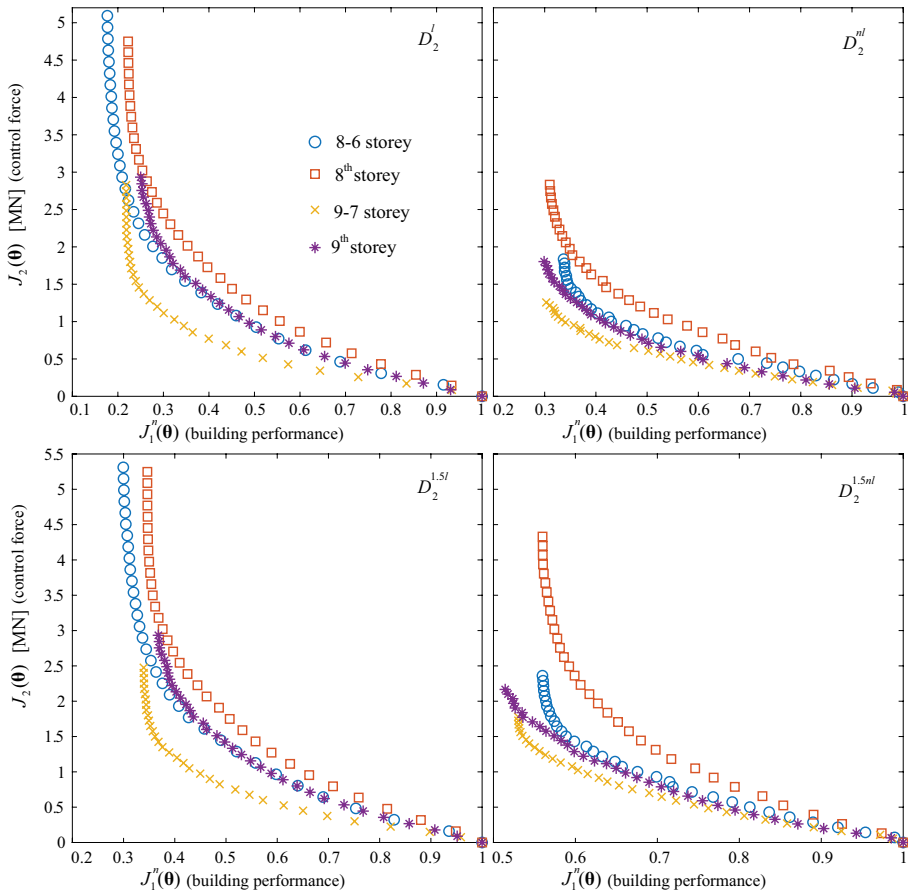
Fig. 9 Pareto front for acceleration-sensitive design (consequence quantification O_2 ), for linear (left) and nonlinear (right) structural behavior, for scaling of intensity s_c = 1 (top row) and s_c = 1.5 (bottom row)
