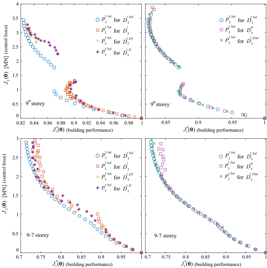
Fig. 13 Performance assessment for the nonlinear structure and for high seismic intensity ( s_c = 1.5 ) for balanced consequence quantifications. Optimal Pareto fronts are compared to the performance achieved using linear (left column) or nonlinear (right column) assumption of the structural behavior, each for different seismic intensity scaling cases. Results are presented for 9th storey and 9–7 storey placements
