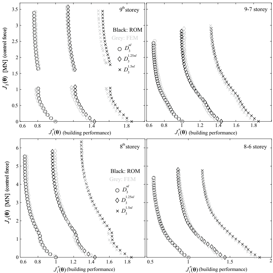
Fig. 4 Comparison between ROM-based optimal design configurations (black color) and their respective FEM-based response predictions (grey color) for the Pareto fronts for balanced design (consequence quantification O_3 ) for the nonlinear structure, for all different scaling factors and for all different protective device placements. Performance for each design is assessed for the nonlinear structure with the corresponding intensity scaling. Normalization of J_1 is established with respect to the uncontrolled structure performance for s_c = 1
