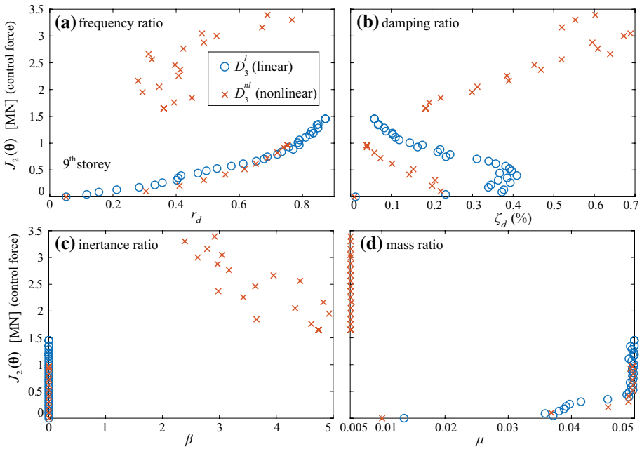
Fig. 7 Design variable values of Pareto optimal solutions plotted against objective J_2 (protective device force) for balanced design, and 9th-storey device placement, for both the linear and nonlinear structure
