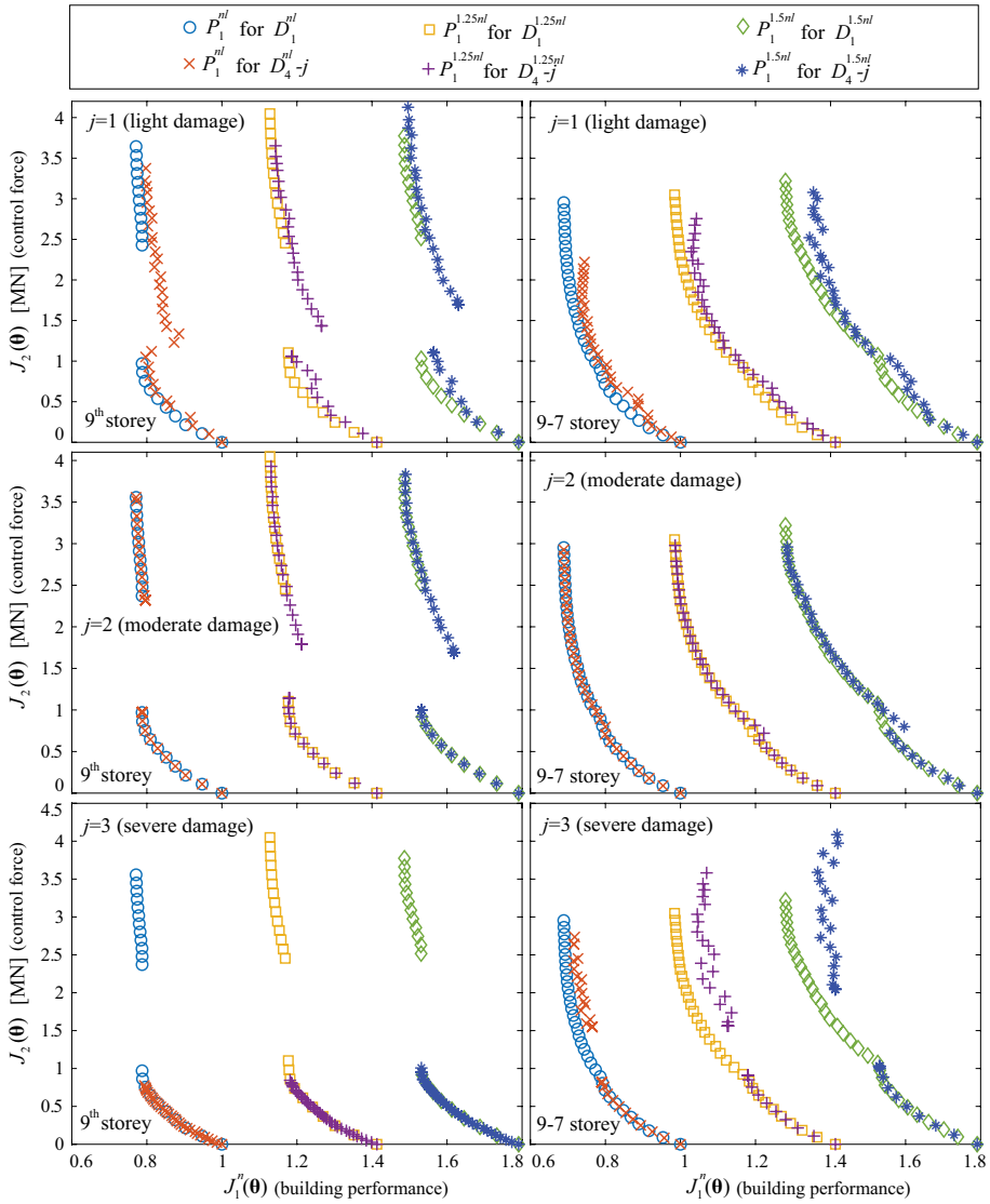
Fig. 14 Performance assessment for the nonlinear structure and for different seismic intensities for drift-sensitive consequence quantification. Optimal Pareto fronts are compared to the performance achieved by designs utilizing O_4 - j consequence quantifications for three different values of j (rows), corresponding to emphasis on light ( j=1 ), moderate ( j=2 ) or severe ( j=3 ) damage states at the design. Results are presented for 9th storey (left column) and 9–7 storey (right column) placements. Normalization of J_1 is established with respect to the uncontrolled structure performance for s_c=1 and for the O_1 consequence quantification
