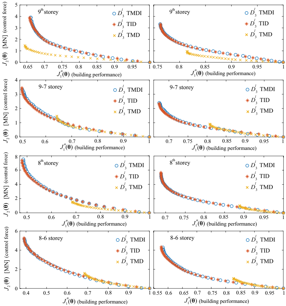
Fig. 5 Pareto fronts for each of the three protective devices, for balanced design (consequence quantification O_2 ) for both the linear (left column) and nonlinear structure (right column), for scaling factor s_c = 1 and for all different protective device placements. Performance for each design is assessed for the corresponding (to the design implemented) linear or nonlinear structure and intensity scaling
