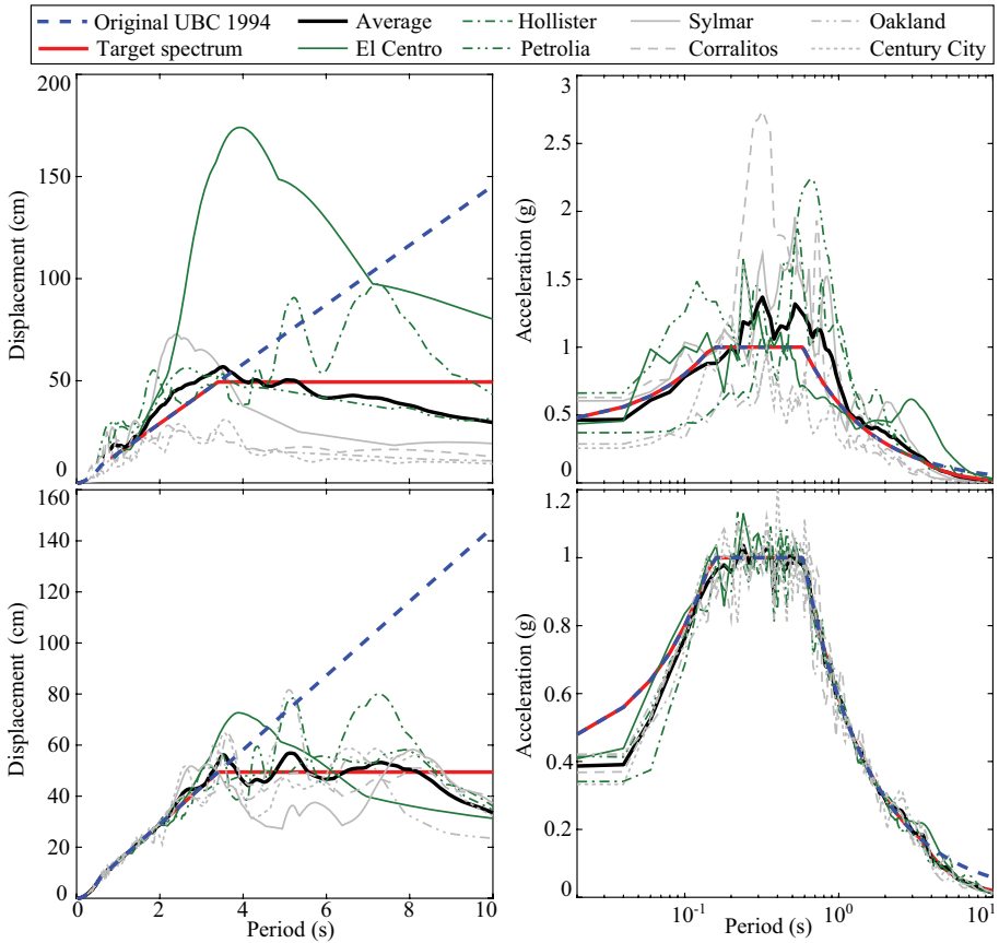
Fig. 2 Response spectra (displacement and acceleration) of the original (top row) and modified (bottom row) GMs
