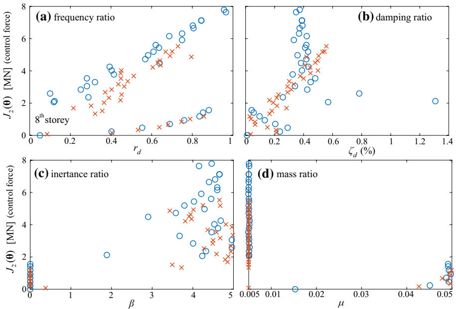
Fig. 8 Design variable values of Pareto optimal solutions plotted against objective J_2 (protective device force) for balanced design, and 8th-storey device placement, for both the linear and nonlinear structure
