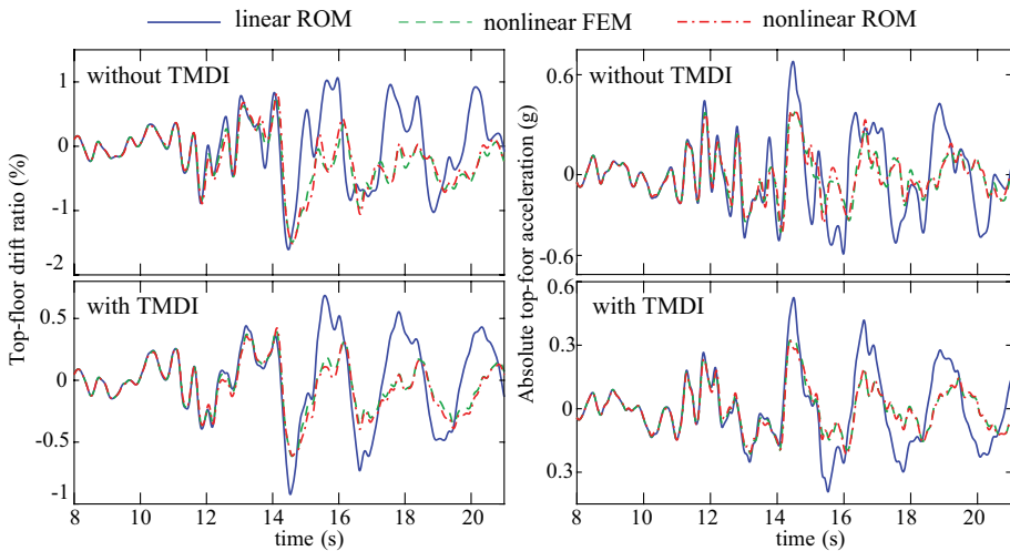
Fig. 3 Time-history responses for top-floor drift ratio (left column) and top-floor acceleration (right column), for the Sylmar ground motion and for the case without TMDI (top row) and with a TMDI (bottom row)
