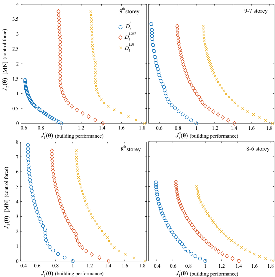
Fig. 6 Pareto fronts for balanced design (consequence quantification O_3 ) for the linear structure, for all different scaling factors and for all different protective device placements. Performance for each design is assessed for the linear structure with the corresponding intensity scaling. Normalization of J_1 is established with respect to the uncontrolled structure performance for s_c = 1
