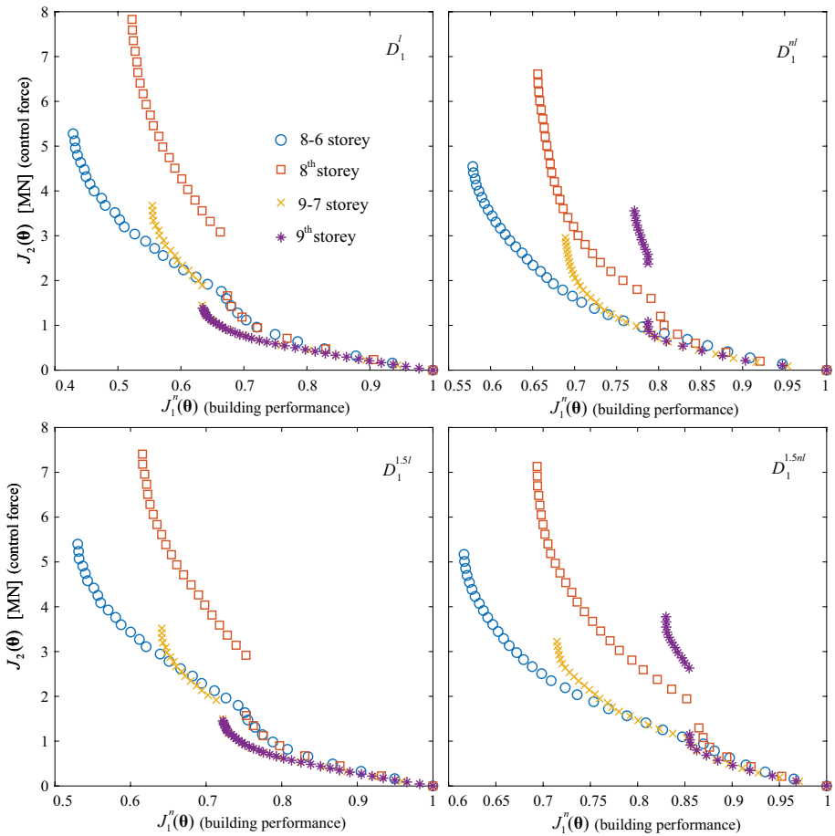
Fig. 10 Pareto front for drift-sensitive design (consequence quantification O_1 ), for linear (left) and nonlinear (right) structural behavior, for scaling of intensity s_c = 1 (top row) and s_c = 1.5 (bottom row)
