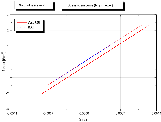
Fig. 22 Stress–strain relationship of the steel columns of the right building for Case (2) under the Northridge earthquake
