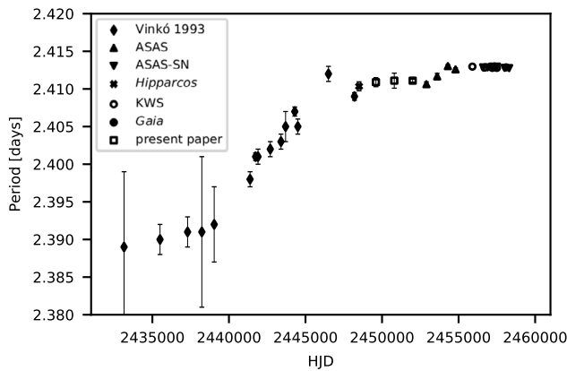
Fig. 7 The pulsation period of AU Pegasi as a function of time
