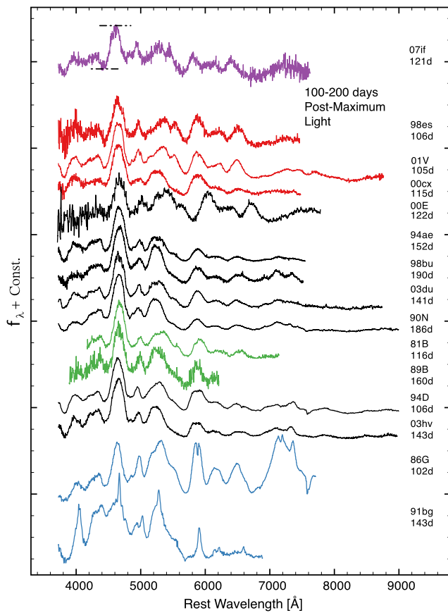
Fig. 12 100+ days post-maximum light optical spectroscopic comparisons. See Fig. 5 caption
