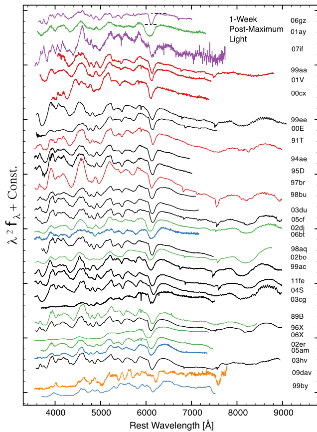
Fig. 8 1-Week post-maximum light optical spectroscopic comparisons. See Fig. 5 caption
