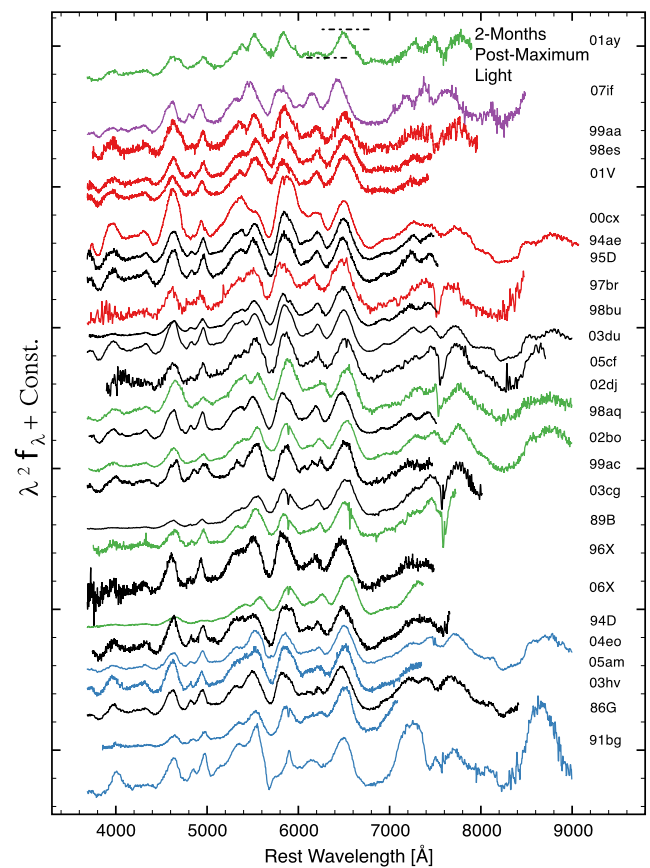
Fig. 11 2-Months post-maximum light optical spectroscopic comparisons. See Fig. 5 caption
