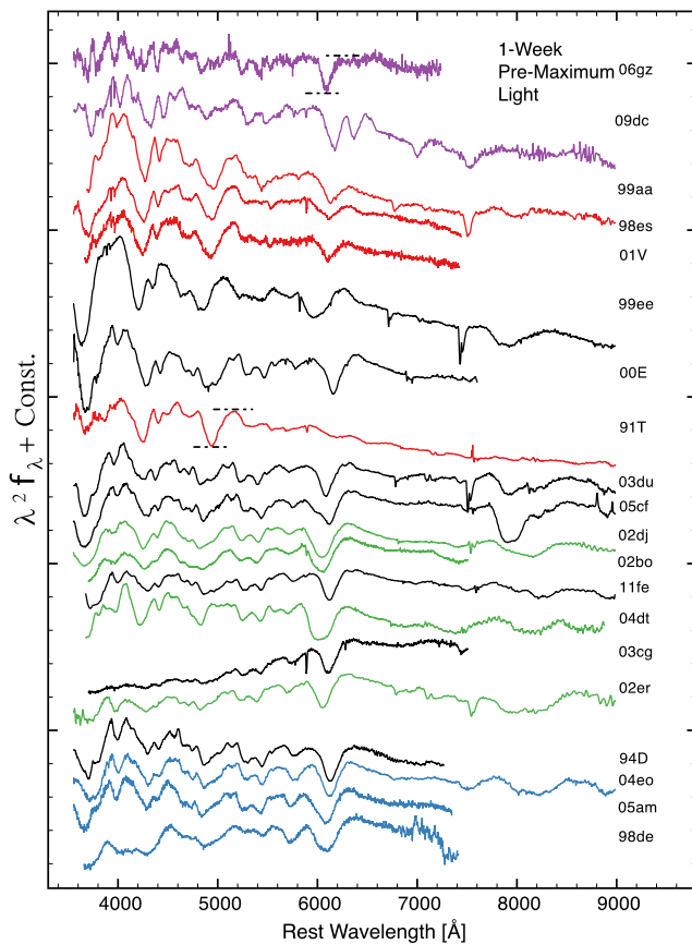
Fig. 6 1-Week pre-maximum light optical spectroscopic comparisons. See Fig. 5 caption
