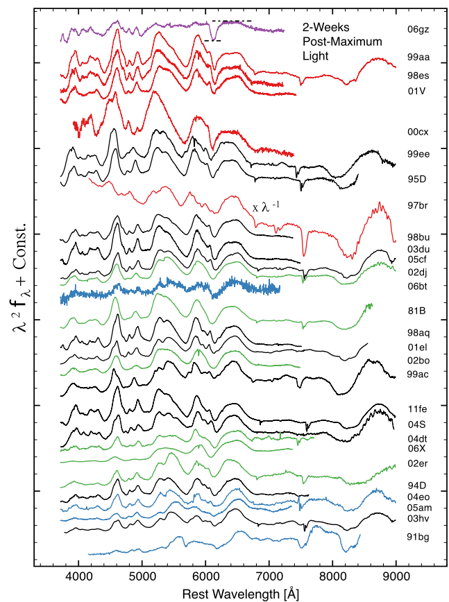
Fig. 9 Two weeks post-maximum light optical spectroscopic comparisons. See Fig. 5 caption
