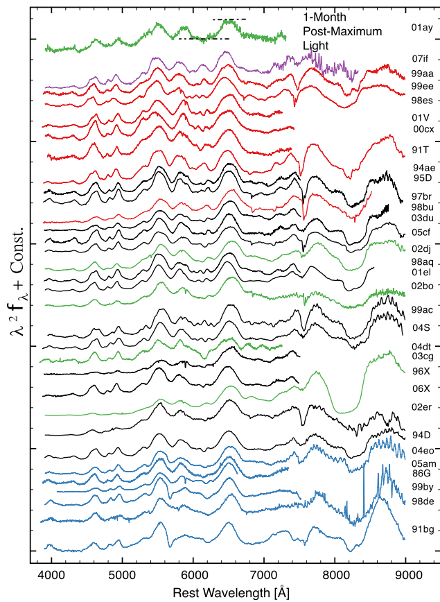
Fig. 10 1-Month post-maximum light optical spectroscopic comparisons. See Fig. 5 caption
