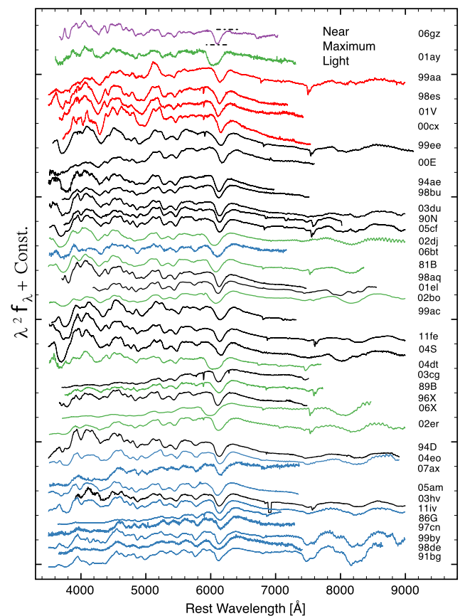
Fig. 7 Maximum light optical spectroscopic comparisons. See Fig. 5 caption
