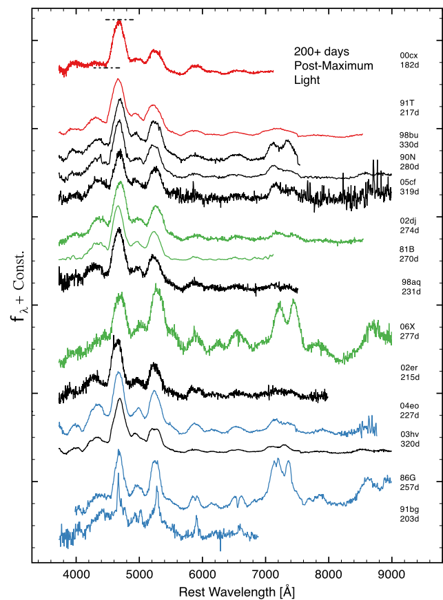
Fig. 13 Late-time optical spectroscopic comparisons. See Fig. 5 caption
