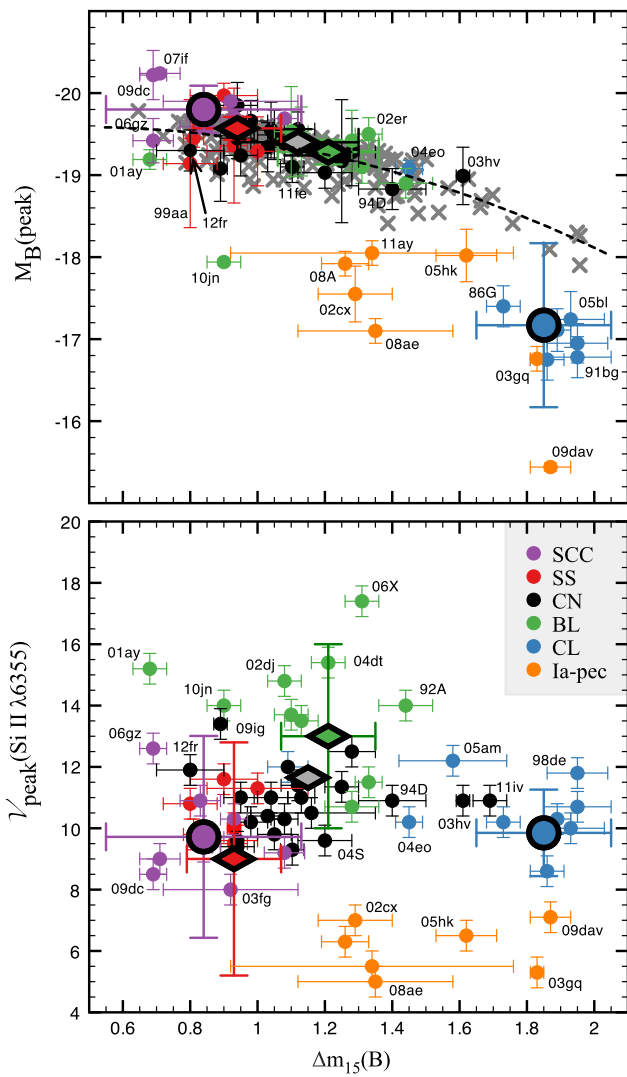
Fig. 14 Top : Peak absolute B -band magnitudes versus \Delta m_{15}(B) for most well-observed SN Ia found in the literature. Additional data (grey) taken from Folatelli et al. (2012), Blondin et al. (2012), and additional points discussed in Pakmor et al. (2013). Bottom : Expansion velocities at maximum light ( \pm 3 days; via Si II \lambda 6355 line velocities) versus \Delta m_{15}(B) . All subtypes have been tagged in accordance with the same color-scheme as in Figs. 5–13. Included for reference are the brightest, peculiar SN 2002cx-likes (light blue circles). Outliers for each subtype have been labeled for clarity and reference. We also plot mean values for the SCC and CL subtypes (larger circles), and include the mean values for SS, CN, and BL SN Ia (large diamonds) as reported by Blondin et al. (2012)
