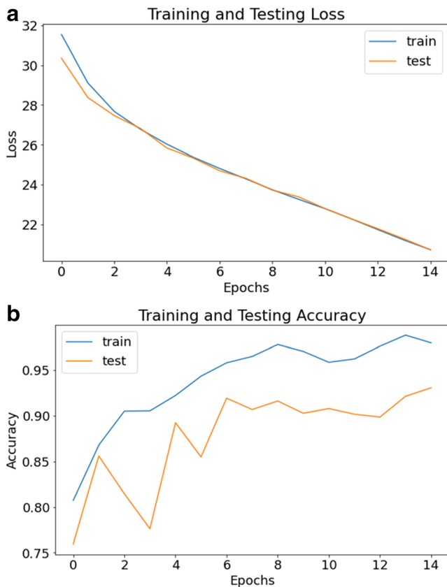
Fig. 9 (a) Training and Testing Loss of ResNeXt model. (b) Training and Testing Accuracy of ResNeXt model
