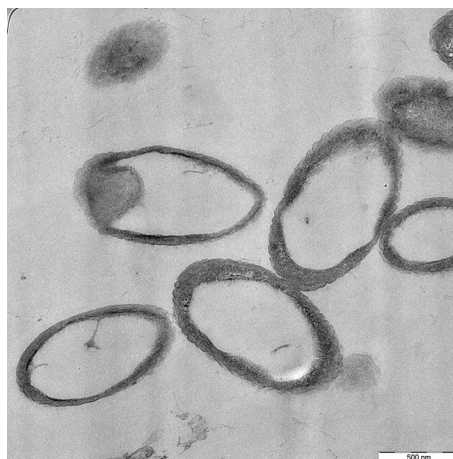
Fig. 1 Transmission electron micrograph of Cupriavidus malaysiensis USMAA1020 T grown in MSM containing \gamma -butyrolactone for 48 h through one-stage cultivation. Bar represents 500 nm
