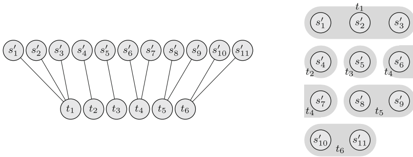
(a) A feasible matching for d = 4 . The indices of the nodes correspond to the first step of the construction described in the proof. In this case, k = 2 and r = 3 .
