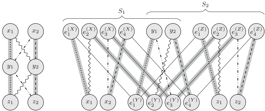
(a) An instance of the 3-dimensional matching problem. (b) The corresponding instance of the double matching problem.
