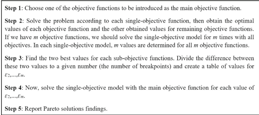
Fig. 9 Execution steps of the proposed \epsilon -constraint
