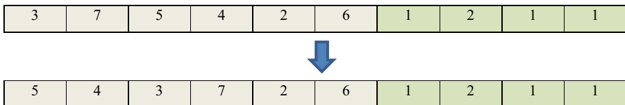
Fig. 5 An example of seed reputation in MOIWOA
