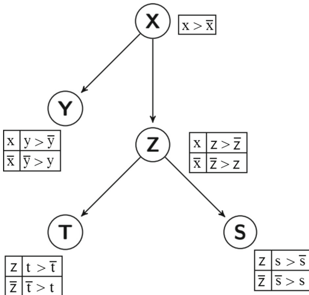
Fig. 1 CP-net associated to Example 1
