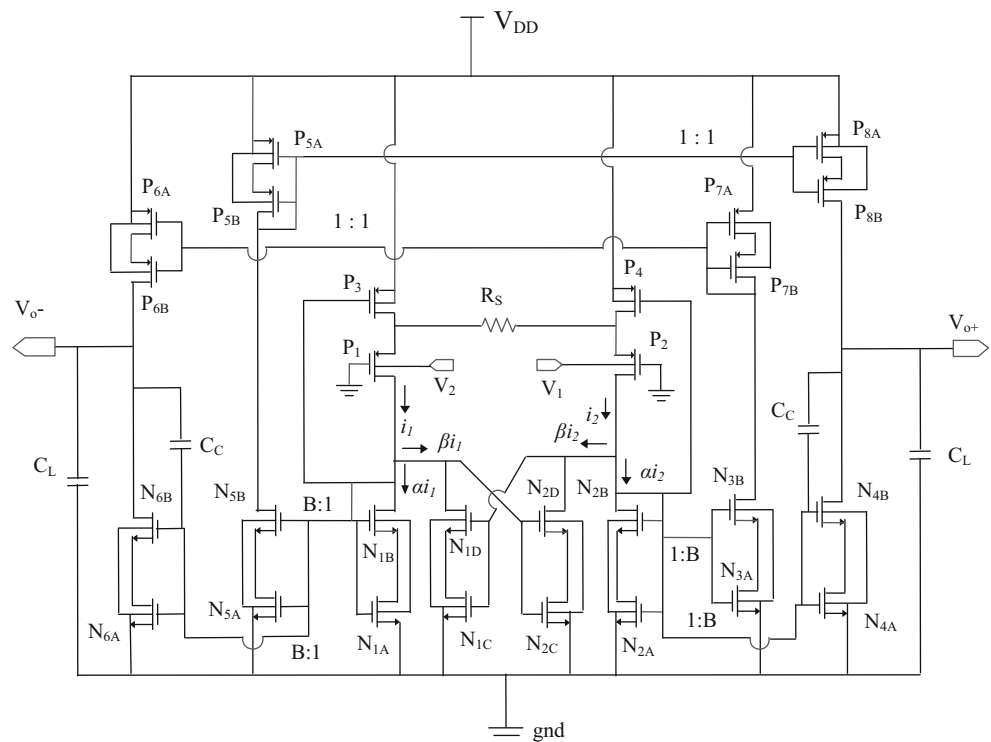
Fig. 3 The subthreshold FD-OTA, having bulk-driven FVF input core with partial positive feedback and current mirror self-cascode load
