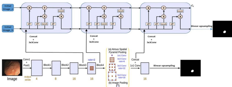
Fig. 7 DeepLab_v3 and LSTM parallel modules (Xiao et al. 2018)
