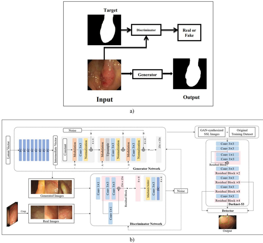
Fig. 18 a Conditional GANs polyp segmentation architecture (Poorneshwaran et al. 2019), b GAN is used to build an automated polyp segmentation system with SSL enhancement. “A” denotes a learned affine transform in the generator network, while “B” controls the noise broadcast (Yoon et al. 2022)
