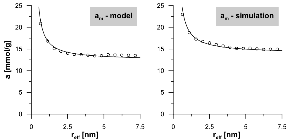
Fig. 5 The dependence between monolayer capacity and tube radius for SWNTs; left panel —monolayer capacity from the model (equations (7) and (10)); right panel —monolayer capacity estimated from simulations for p/p_s = 1 ; solid line —theoretically predicted values from (16) (from the model— a_m^{(g)} = 12.41 mmol/g and from simulation— a_m^{(g)} = 13.97 mmol/g)
