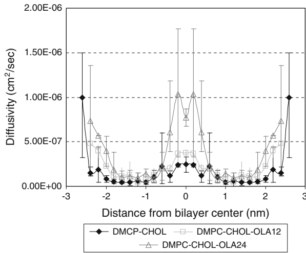
FIGURE 5. Lateral diffusivities of fentanyl in dmcp-cholesterol (filled) and dmpc-cholesterol-oleic acid (open) bilayers as functions of depth.
