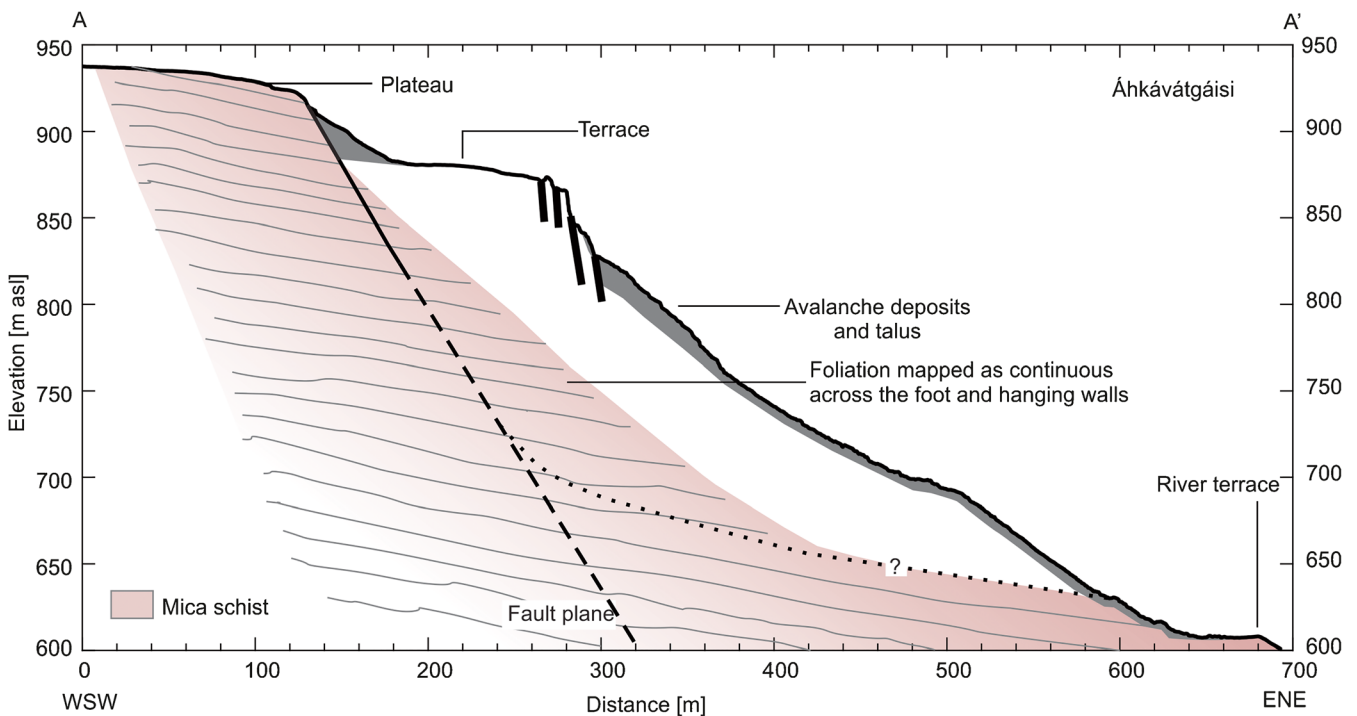
Fig. 29 A–A' cross section of Áhkávátgáisi, based on 0.5 m DEM (location on Fig. 28), showing exposed fault plane in the backscarp. Mapped rupture planes indicated by heavy black lines, and inferred rupture planes indicated by a dashed line. Fault trace after Bunkholt et al. (2013a). Geology from Quenardel and Zwaan (2008)
