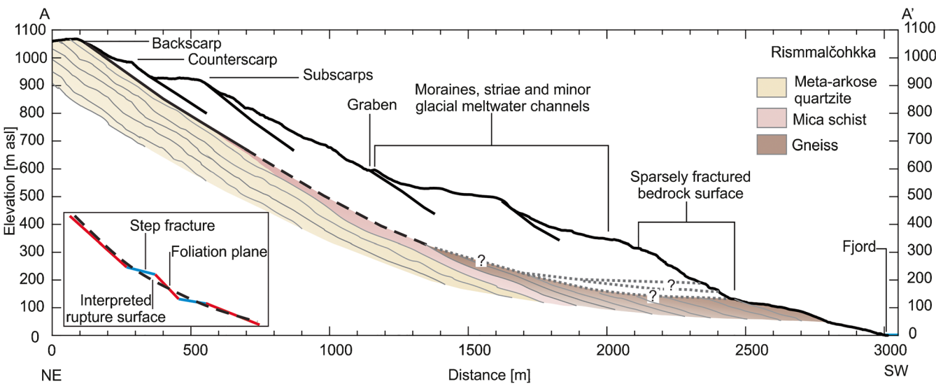
Fig. 8 A–A’ cross section of Rismmalčohkka, based on 0.5 m DEM (location on Fig. 7), showing exposed foliation-parallel sliding surfaces. Mapped rupture surfaces indicated by heavy black lines, inferred rupture planes indicated by a dashed line, uncertain rupture surfaces by a dotted line. Inset is showing structural configuration of the rupture plane. Glacial geomorphology is based on Tolgensbakk and Sollid (1988) and geology on Zwaan et al. (2006)
