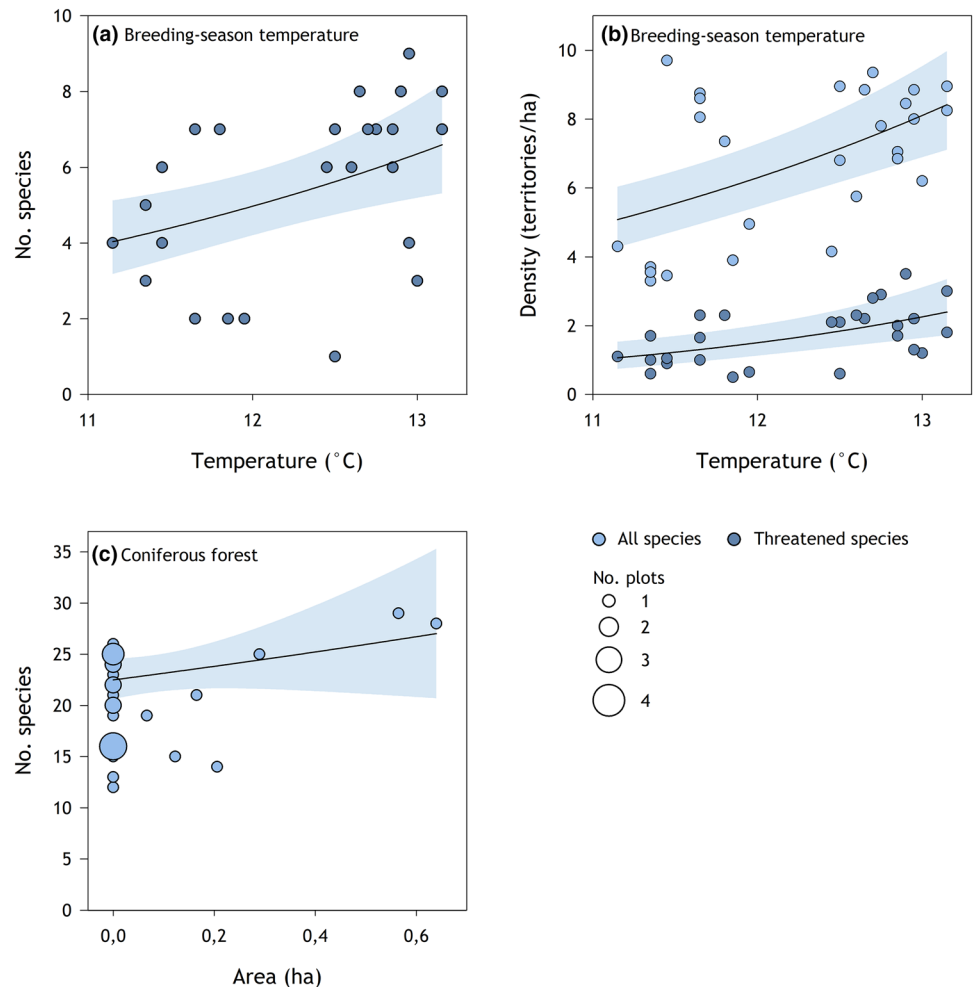
Fig. 5 Relationship between species richness and density of all and threatened breeding-bird species, respectively, and the significant environmental parameters of averaged models for plots of mesic grasslands ( N=27 ) (see Table 4). The regression slopes (including 95% confidence intervals) were fitted using a single predictor GLMM (negative binomial error structure)
