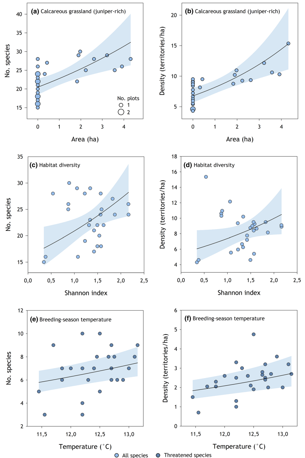
Fig. 4 Relationship between species richness and density of all and threatened breeding bird species, respectively, and the significant environmental parameters of averaged models for plots of calcareous grasslands ( N=27 ) (see Table 3). The regression slopes (including 95% confidence intervals) were fitted using a single predictor GLMM (negative binomial error structure)
