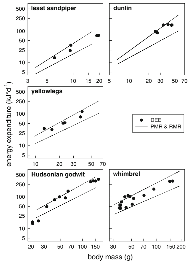
Fig. 3 Daily energy expenditure ( symbols ) as a function of body mass, in relation to peak and resting metabolic rate (PMR and RMR, lines ) in chicks of different species of shorebirds. PMR and RMR are shown as regression lines calculated as described in Williams et al. (2007)
