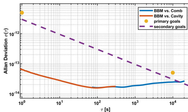
Fig. 8 Frequency instability of the BBM, given as Allan deviation for a given timespan \tau . The measured short-term stability (red, measured against an ultra-stable cavity) is almost two orders of magnitude higher than the primary (yellow dots) and secondary (purple dashed line) goals of the COMPASSO mission for short times. The long-term performance (blue, measured against a comb locked to a maser) meets the requirements up to an integration times of around 10^4 s
