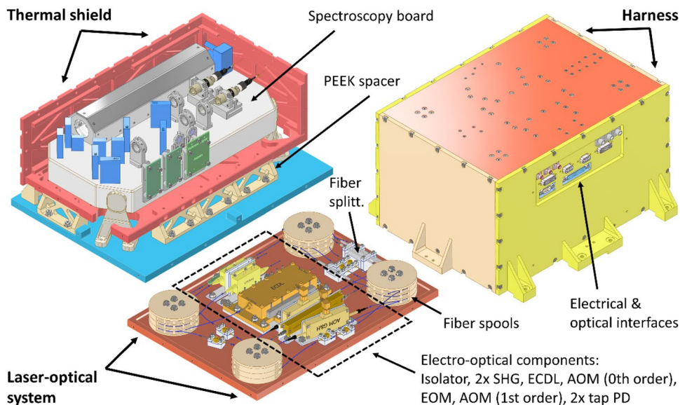
Fig. 6 CAD model of the iodine spectroscopy unit (ISU). The spectroscopy board is encapsulated by the heat shield indicated with red color (top left). The laser-optical system (bottom) is mounted beneath the cover plate of the ISU (orange). The electro-optical components are indicated by the dashed rectangle with the labeling from top left to bottom right. The closed harness is depicted on the top right side. The yellow side plate hosts all electrical connectors to power and control the ISU
