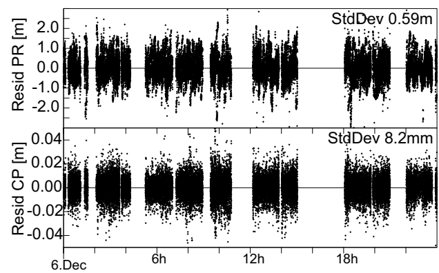
Fig. 7 Code and carrier phase residuals for the ionosphere-free dual-frequency combination obtained in a precise orbit determination with the GPS-2 antenna and receiver of CASSIOPE on December 6, 2018
