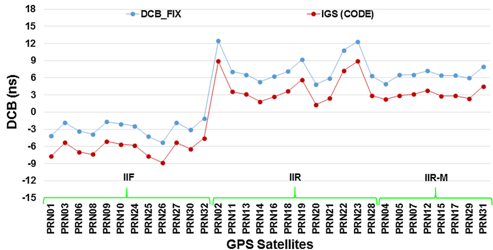
Fig. 6 Plot showing the average GPS satellite DCBs between P1 and P2 estimated by the DCB_FIX software (SEPT = -4.41 ns) and IGS (CODE) over a period of 22 days (March 17 to April 7, 2016)
