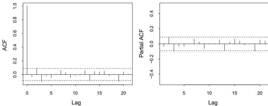
Fig. 4 Autocorrelation and partial autocorrelation functions for the deviance residuals of the estimated GAM beta regression in Table 1
