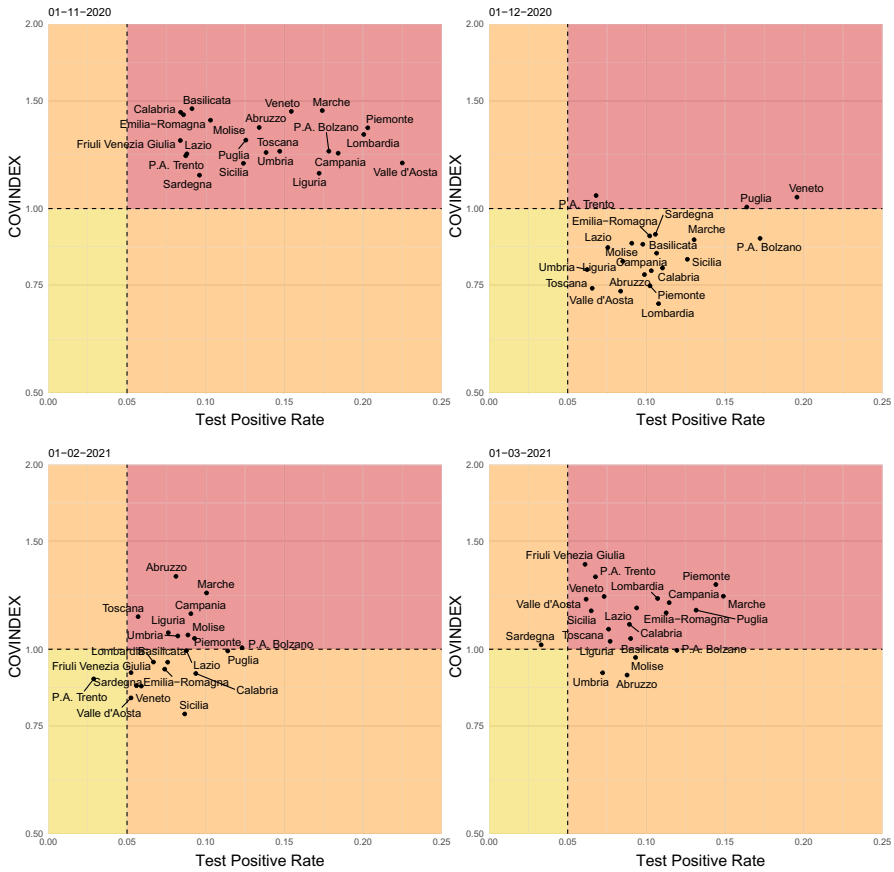
Fig. 10 TPR-COVINDEX plot for Italian regions at different time points
