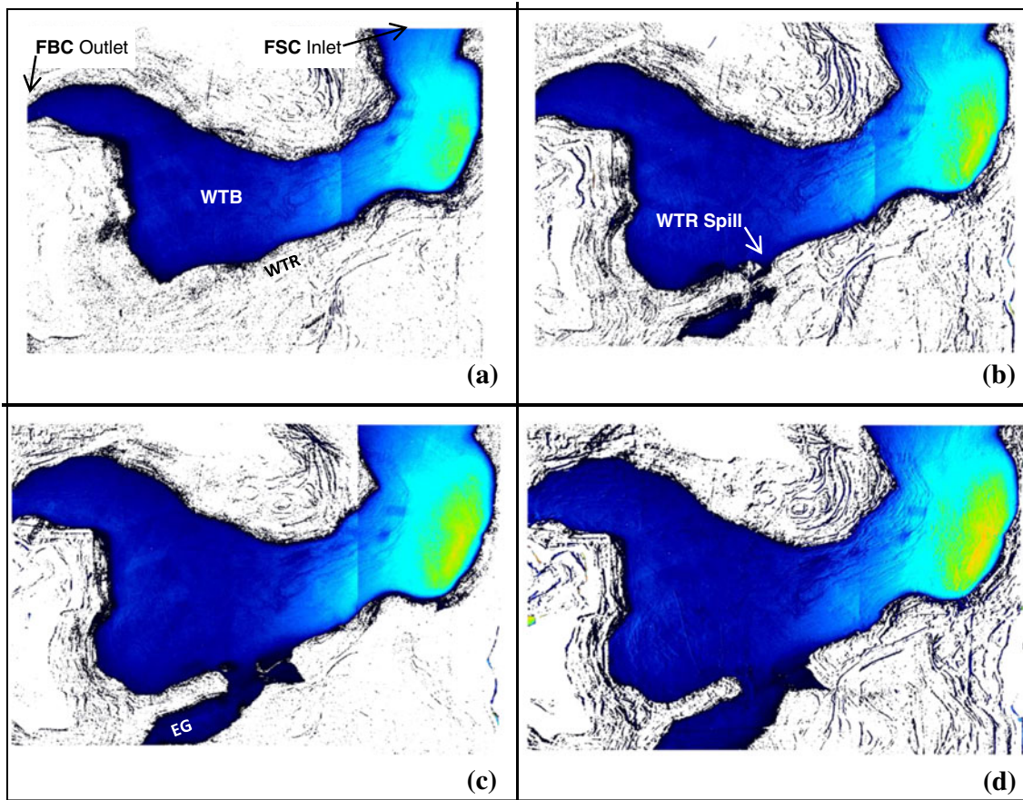
Fig. 4 Dense bottom-water overflow pathways observed through illuminated fluorescense dye-tracing for run 1 conditions (see Table 1) with Bu_1: Q_1^* values of a 0.124:0.00352 (no WTR spill), b 0.116:0.00528 (WTR spill), c 0.114:0.00704 (WTR spill) and d 0.115:0.00915 (WTR spill)
