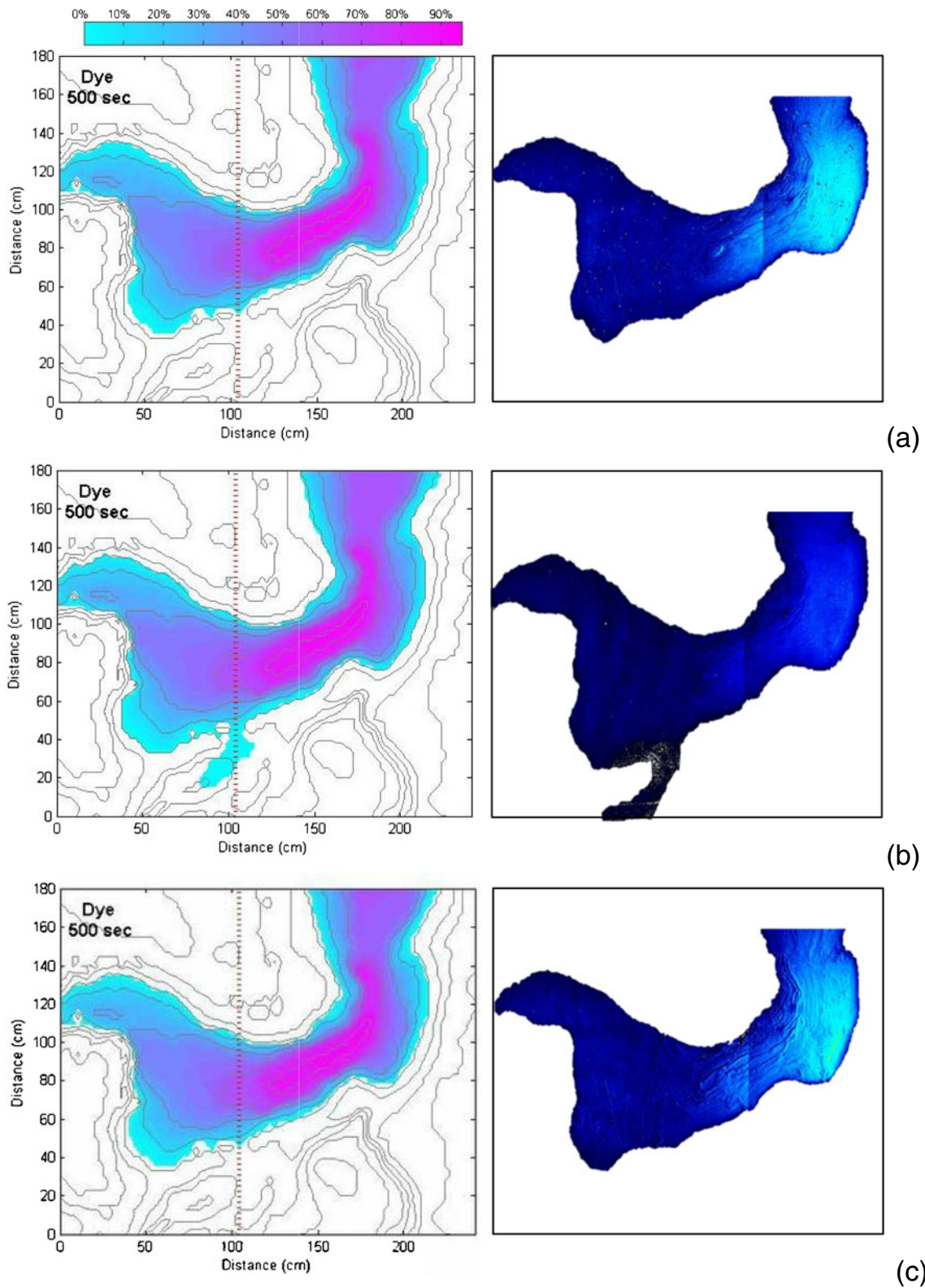
Fig. 10 Comparison of MITgcm-predicted ( left ) and measured ( right ) dyed bottom-water traces through Faroese channel topography for Bu_1: Q_i^* values of a 0.363:0.00019 (run 3b; Table 1), b 0.202:0.00126 (run 2c)
