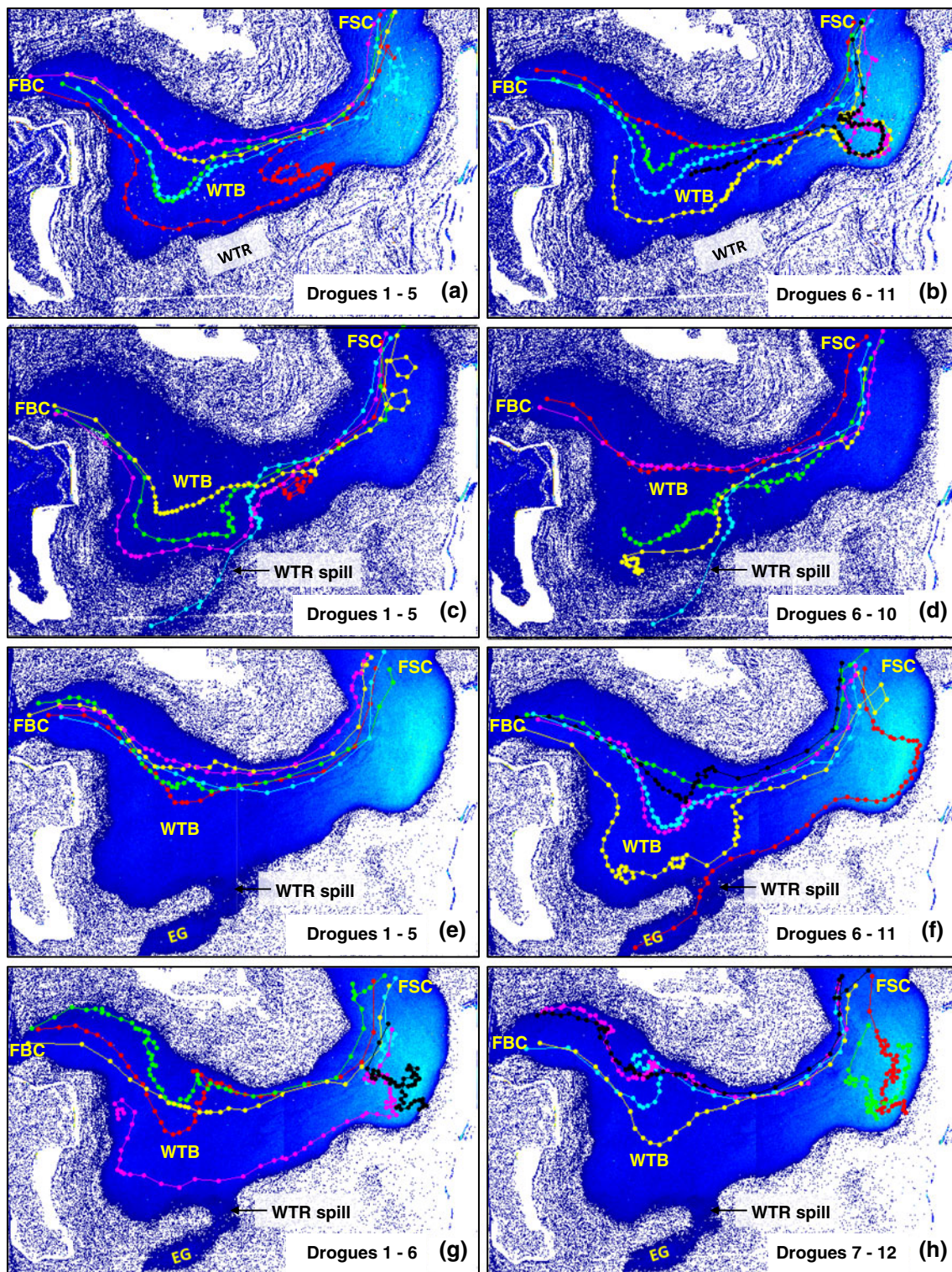
Fig. 6 Typical drogue tracking for dense water outflow layer in Faroese Channels region under investigation for runs with Bu_1 : Q_1^* values of a–b 0.363:1.9 \times 10^{-4} (run 3b, Table 1); c–d 0.202:1.26 \times 10^{-3} (run 2c); e–f 0.114:5.99 \times 10^{-3} (run 5c); g–h 0.110:4.49 \times 10^{-3} (run 5b). Time step between
