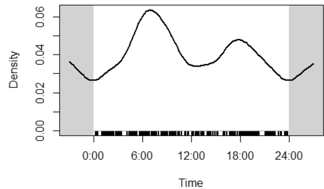
Fig. 1 Density plot of jaguar activity from camera trap data. Original records presented as a rug along the “time” axis
