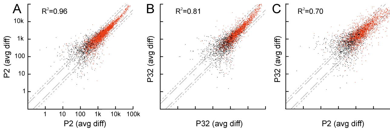
FIG. 1. Scatter plots showing the correlation of expression patterns. A Two P2 samples compared with each other. B Two P32 samples. C A P32 sample compared with a P2 sample. Average difference values (Avg Diff determined by the analysis software) were used to quantify expression and were plotted on a log scale. The correlation coefficient between samples ( R^2 ) is also shown for each comparison. The dashed gray line demarcates less than twofold difference be-
