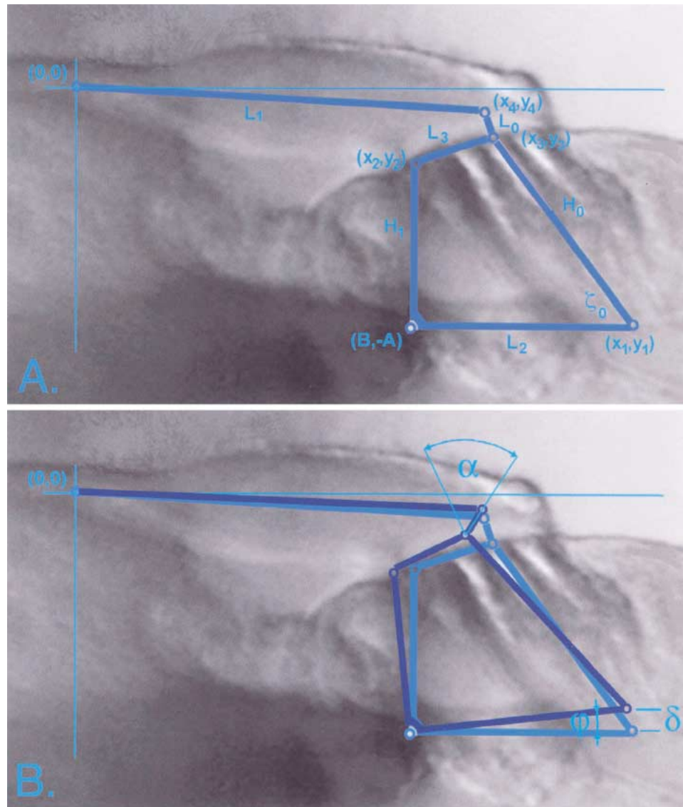
FIG. 1. Hemicochlea image of organ of Corti and tectorial membrane (TM) with critical elements represented as rigid, hinged beams. A Coordinate system is placed with its origin at the hinge point of the TM at the spiral limbus. Organ of Corti frame rotates around a hinge point (B,-A) where the basilar membrane (BM) meets the osseous spiral lamina. Combined pillar cells are represented by the beam H_1 , perpendicular to the BM and rigidly tied to it. Three rows of OHCs and Deiters' cells are collapsed into a single beam ( H_0 ), hinged to the BM at the location of the second row of OHCs and also to the reticular lamina ( L_3 ). B indicates how the frame rotates when the BM displacement at the point of the attachment of H_0 is \Delta . The BM, rotating as a rigid beam around its insertion point, subtends an angle Z when the BM is displaced by \Delta . The result of this displacement is a change in cilia angle from its resting 90^\circ to \alpha .
