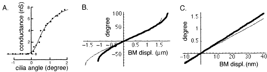
FIG. 3. A. Transducer conductance as a function of cilia displacement angle (modified from Kros et al. 1995). B. Basal turn response is replotted (heavy line) from Figure 2A, along with the results of an approximate computation (thin line); see text. C. A restricted portion of the curves from B is shown to correspond to the dynamic range of cilia deflections as gleaned from A .
