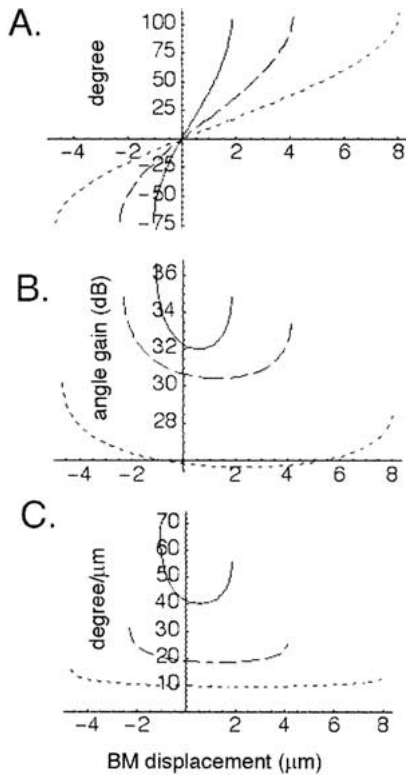
FIG. 2. Computational results for three cochlear locations using the parameters listed in Table 1. A. Cilia angle change ( \alpha in degrees) in response to BM displacement ( \Delta in micrometers). B. Ratio of cilia angle and basilar membrane angle ( \alpha/Z , expressed in decibels). C. Ratio of cilia angle and BM displacement ( \alpha/\Delta , expressed in degrees/micrometer).
