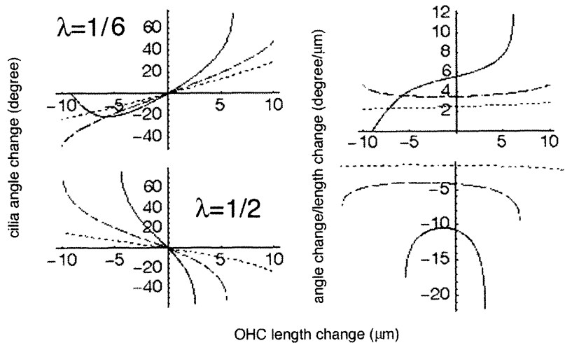
FIG. 4. Computational results for the case where excitation is due to OHC length changes. Left column: cilia-angle change ( \alpha in degrees), right column: cilia-angle change divided by OHC length change ( \alpha/d in degrees/micrometer). Two cases are shown. On the top, the RL moves five times the displacement of the BM. This corresponds to the measurements of Mammano and Ashmore (1993). On the bottom, computational results are shown for equal motion of BM and RL.
