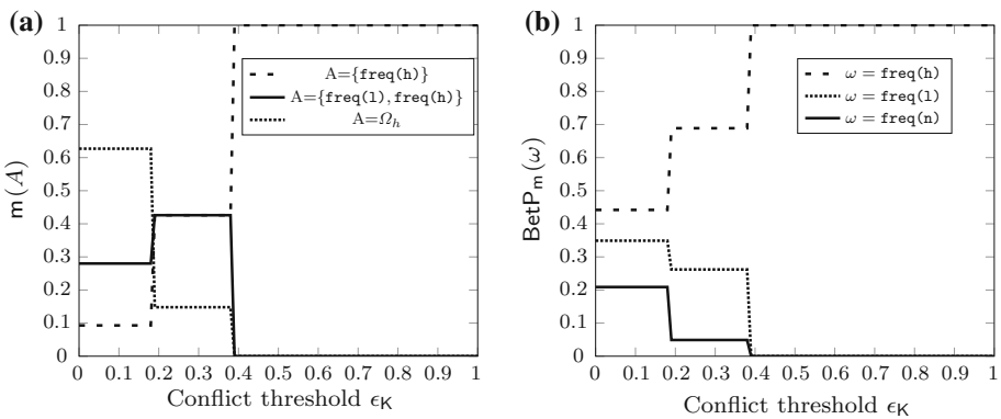
Fig. 1 Effect of varying the conflict threshold on m(A) and BetP_m(\omega) . a Effect of conflict threshold on m(A) , b effect of conflict threshold on BetP_m(\omega)
