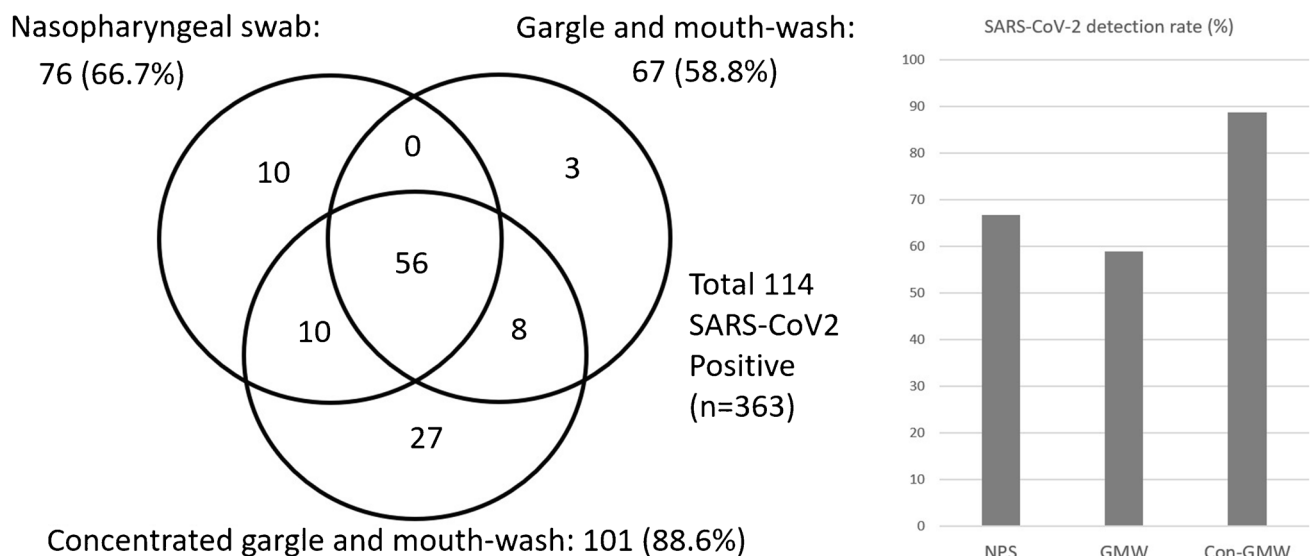
Fig. 2 Detection of SARS-CoV-2 RNA, by RT-PCR in nasopharyngeal swab samples, in gargle and mouthwash samples, before and after concentration by MyMagiCon-RW100 ®
