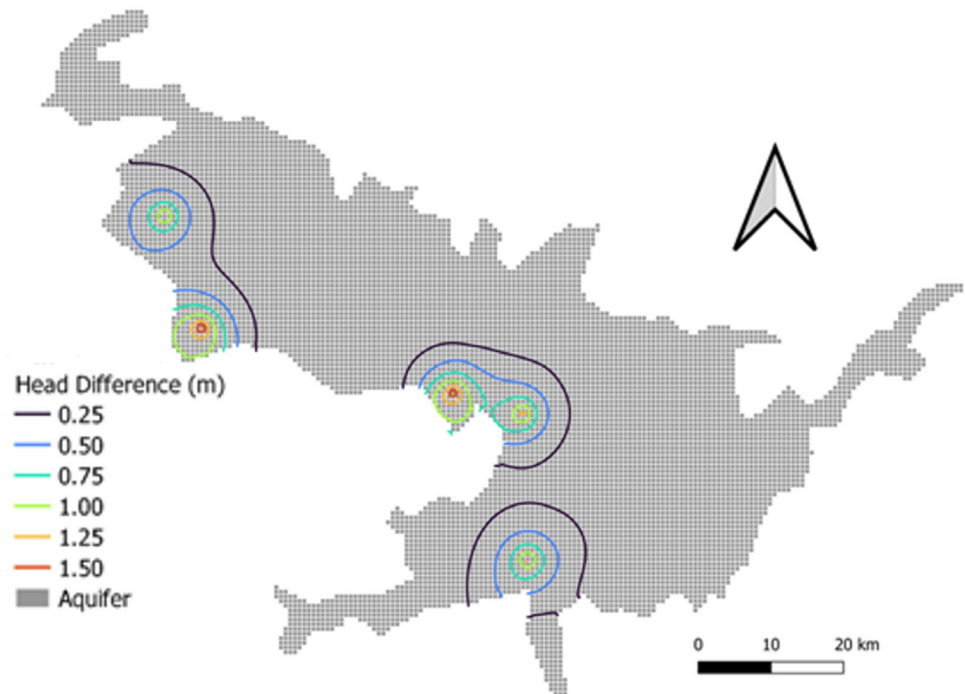
Fig. 14 The head difference (m) between the simulation with CAC active and without CAC at the end of simulation, considering a streambed hydraulic conductivity of 2.21 m/day
