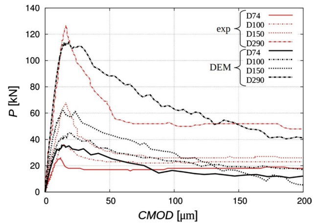
Fig. 14 Vertical force P against crack mouth opening displacement (CMOD) from experiments by Carmona et al. [34] (red lines) as compared to DEM (black lines) for different specimen diameters ( D=74 mm (D74), D=100 mm (D100), D=150 mm (D150) and D=290 mm (D290)) (colour figure online)
