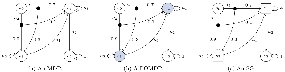
Fig. 2 Examples of a classical MDP, POMDP, and SG
