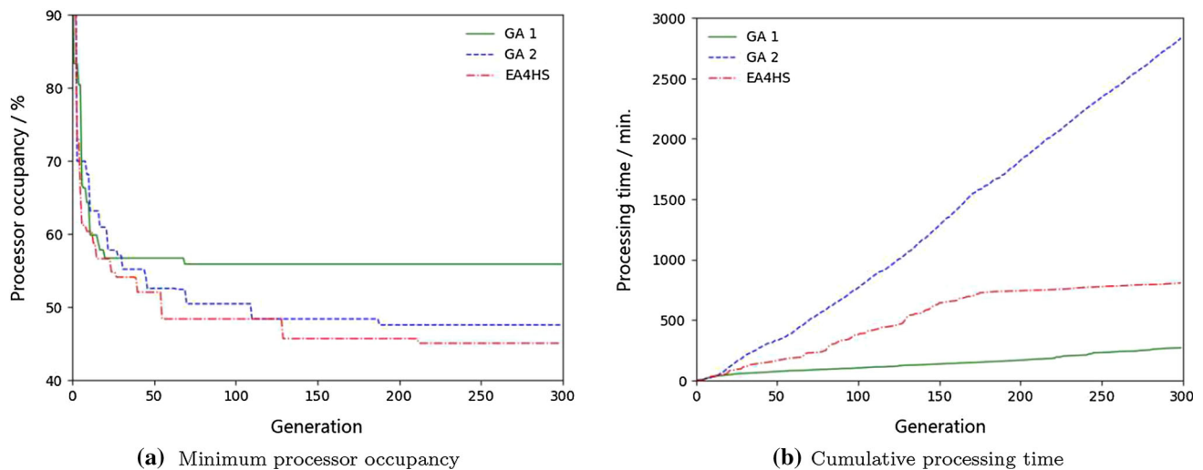
Fig. 10 Evolution of minimum processor occupancy and cumulative processing time in Experiment 2
