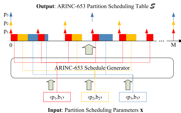
Fig. 4 Data flow of an ARINC-653 schedule generator
