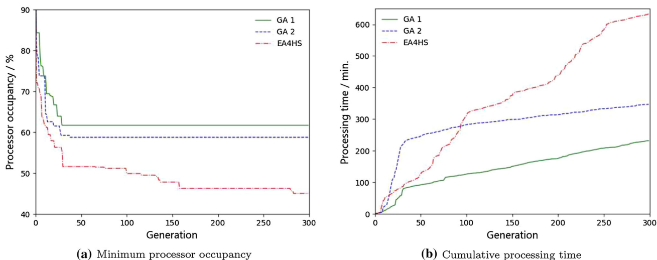
Fig. 9 Evolution of minimum processor occupancy and cumulative processing time in Experiment 1
