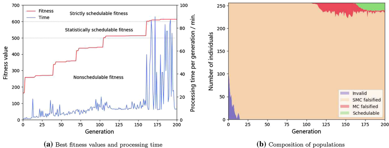
Fig. 11 Evolution of best fitness values, processing time and population composition in Experiment 3
