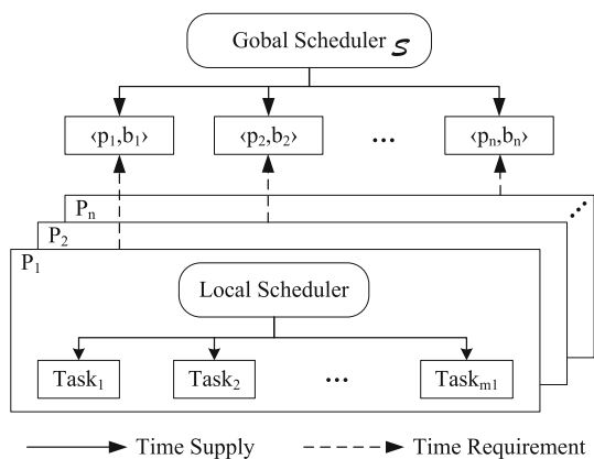
Fig. 1 Hierarchical architecture of partitioned scheduling systems
