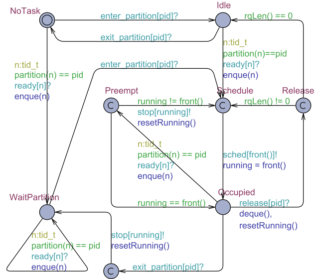
Fig. 5 Local scheduler model
