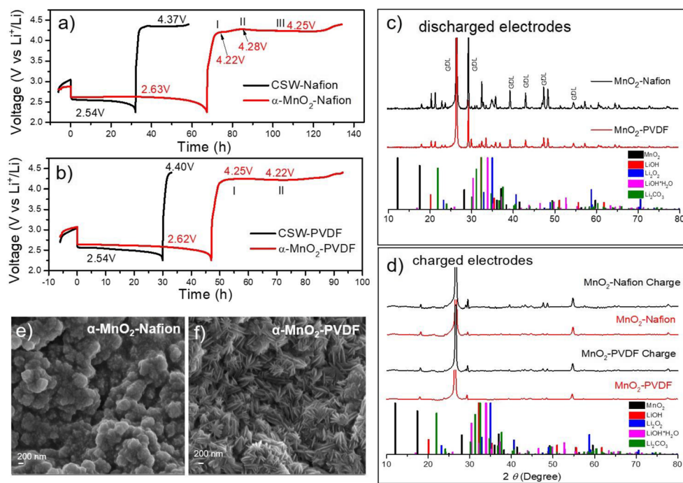
Fig. 2 Discharge/charge profiles of the air electrodes (under 0.1 mA cm -2 current densities and continuously fed by a 3 ml min -1 O 2 flow) with CSW and Nafion against \alpha -MnO 2 and Nafion ( a ), CSW and PVDF against \alpha -MnO 2 and PVDF ( b ), XRD patterns of MnO 2 Nafion and
