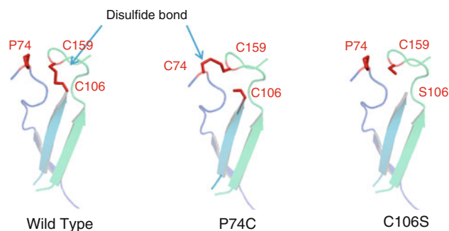
Fig. 3 Comparison of the disulfide bonds from the mutants and wild type. P74C with 3 Cys residues showed an identical disulfide-bonding pattern to EGAc. C106S has no disulfide bond
