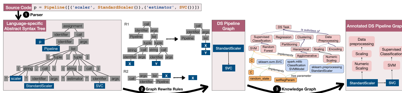
Fig. 4 Extraction of an example DS pipeline from source code. DORIAN parses the textual representation with a language-specific parser, transforms it to a graph with rewrite rules, and semantically enriches the DS graph with a knowledge graph
