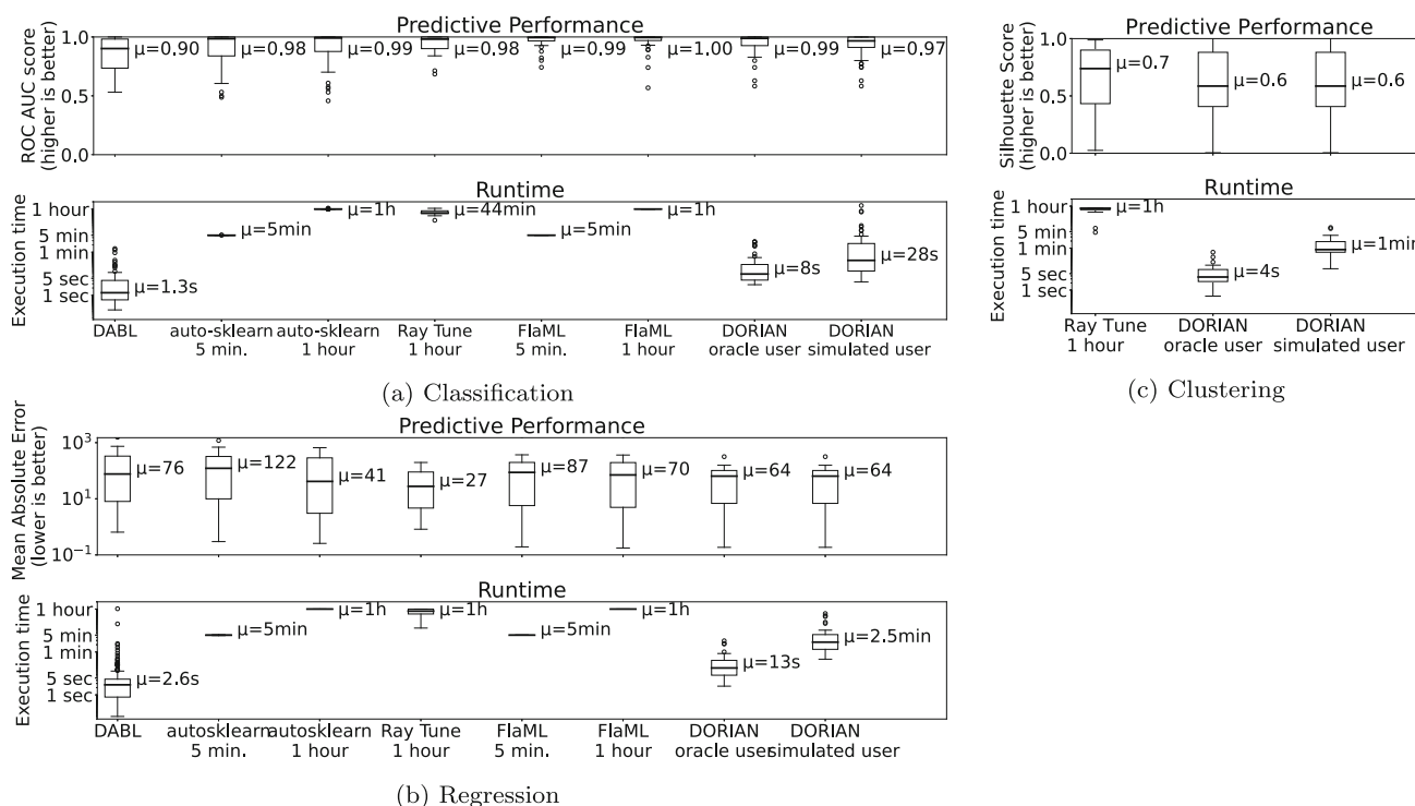
Fig. 5 Comparison against six AutoML baselines: DORIAN performs similarly to its automated counterparts in predictive performance while being significantly faster
