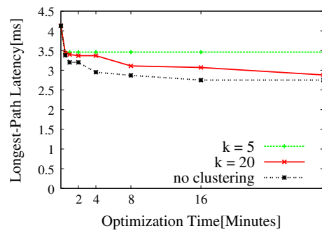
Fig. 9 Convergence for solving LPNDP using MIP. Clustering does not improve performance
