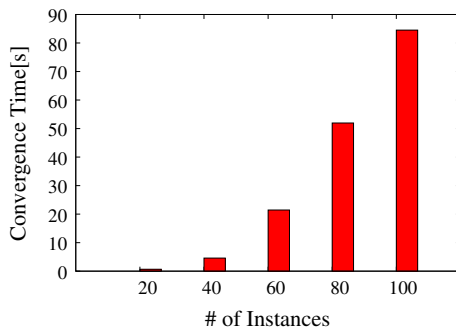
Fig. 8 Scalability for solving LLNDP using CP. Average convergence time increases acceptably with number of instances
