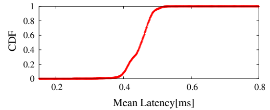
Fig. 18 Latency heterogeneity in Google Compute Engine
