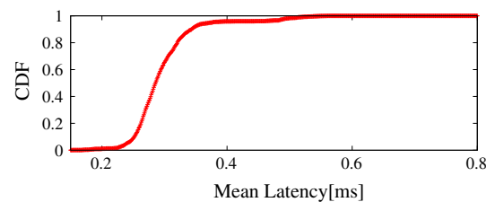
Fig. 20 Latency heterogeneity in Rackspace Cloud Server
