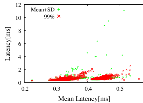
Fig. 10 Correlation between different cost metrics under one representative allocation of 110 instances. The cost metrics are not perfectly correlated with mean latency
