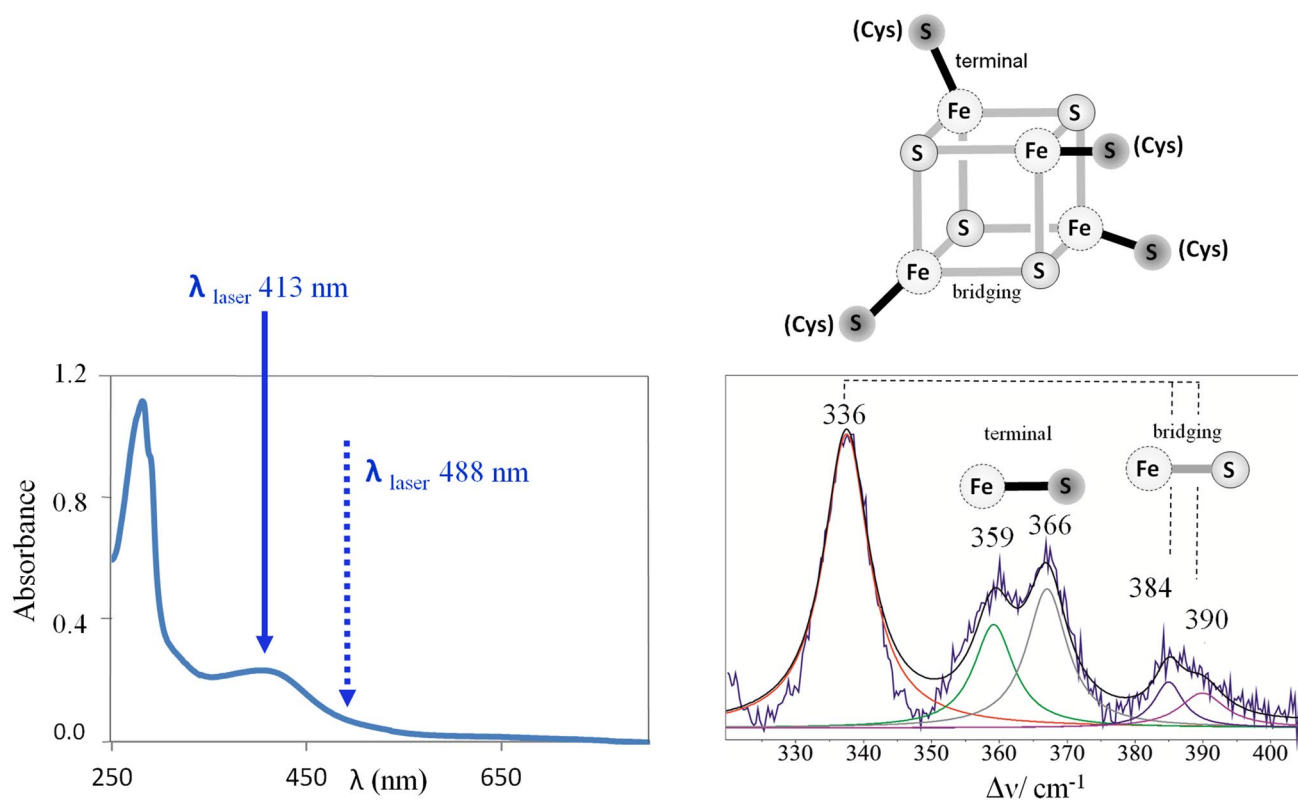
Fig. 1 UV-Vis and RR spectra of a [4\text{Fe-4S}]^{2+} cluster protein. Left panel, UV-Vis spectra with designated laser excitation wavelengths for resonance and pre-resonance enhancement of the signal. Right
