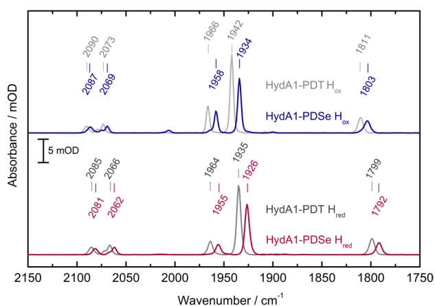
Fig. 2 Comparison of the H_{ox} (gray/blue) and H_{red} (dark gray/red) states of [4Fe-4S]_H HydA1-PDT/-PDSe in FTIR spectroscopy. The smaller contribution at 2005 cm^{-1} in the spectrum of HydA1-PDSe H_{ox} originates from the oxidized CO inhibited state (see Fig. 5). Spectra are taken at 288 K with a spectral resolution of 2 cm^{-1}
