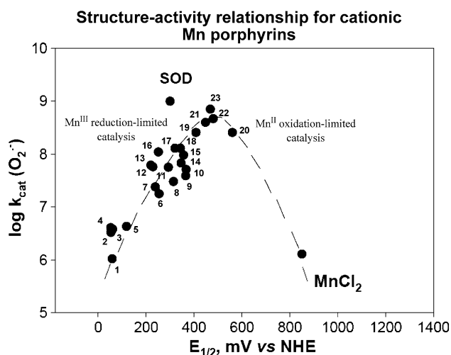
Fig. 3 Structure–activity relationship between \log k_{\text{cat}}(\text{O}_2^{\bullet-}) and E_{1/2} ( \text{Mn}^{\text{III}}\text{P}/\text{Mn}^{\text{II}}\text{P} ) in mV versus NHE for cationic Mn(III) porphyrins. Compounds at the plateau of the bell-shaped curve are those that bear both meso and beta substituents and have highest k_{\text{cat}} . Yet, they are stabilized in Mn +2 oxidation state, lose readily Mn and are thus are only important for mechanistic purposes. The falling limb of the bell-shaped curve is more obvious in SARs of anionic and neutral porphyrins (Batinic-Haberle et al. 2010). Compounds are: 1 MnT(TFTMA)P 5+ , 2 MnBM-2-PyP 5+ , 3 MnTM-4-PyP 5+ , 4 MnTM-3-PyP 5+ , 5 MnTrM-2-PyP 5+ , 6 MnTnBu-2-PyP 5+ , 7 MnTnPr-2-PyP 5+ , 8 MnTnHex-2-PyP 5+ , 9 MnTDMOE-2-ImP 5+ , 10 MnTnOct-2-PyP 5+ , 11 MnCITE-2-PyP 5+ , 12 MnTE-2-PyP 5+ , 13 MnTM-2-PyP 5+ , 14 MnTDE-2-ImP 5+ , 15 MnTM,MOE-2-ImP 5+ , 16 MnTMOE-2-PyP 5+ , 17 MnTDM-2-ImP 5+ , 18 MnCl 2 TE-2-PyP 5+ , 19 MnCl 3 TE-2-PyP 5+ , 20 MnCl 5 TE-2-PyP 5+ , 21 MnCl 4 TE-2-PyP 5+ , 22 MnBr 8 TM-4-PyP 4+ , and 23 MnBr 8 TM-3-PyP 4+ . Data are taken from Batinic-Haberle et al. (2010) and Kachadourian et al. (1998). The names of porphyrins are listed in the list of abbreviations
