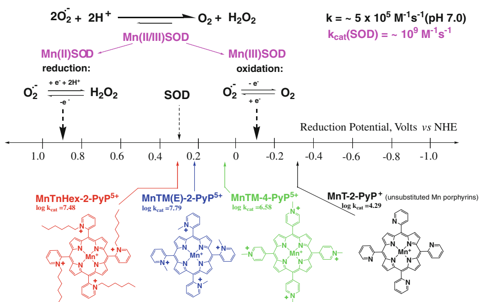
Fig. 1 Design of Mn porphyrins based on thermodynamic considerations
