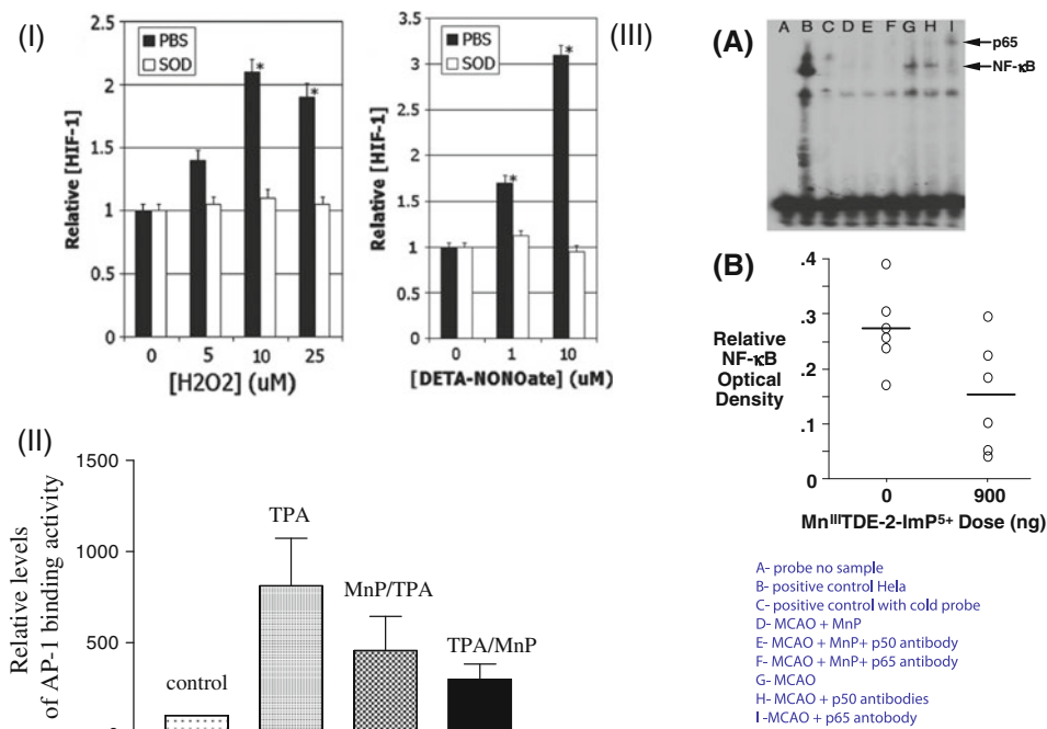
Fig. 5 MnP prevents activation of redox-active cellular transcription factors. In an in vitro 4T1 mouse breast cancer cell study, HIF-1 \alpha was activated by H 2 O 2 and nitric oxide but blocked with equimolar concentrations of MnTE-2-PyP 5+ , indicated in I as SOD (Moeller et al. 2004). In II , the AP-1 activation in a mouse skin cancerogenesis model was inhibited with MnTE-2-PyP 5+ given at 5 ng daily for
