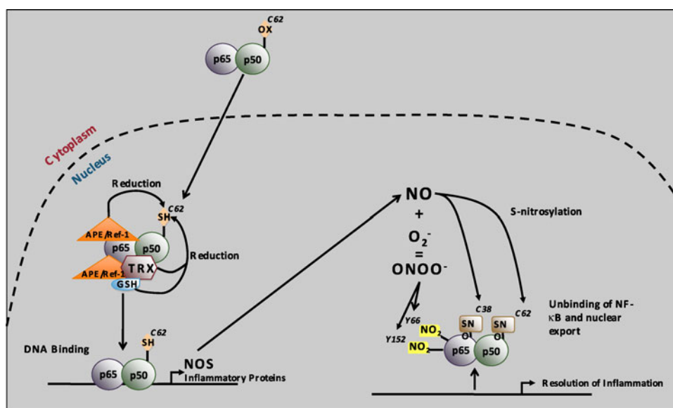
Fig. 6 Redox-regulation of NF- \kappa B DNA-binding. In resting cells, NF- \kappa B is predominantly found in the cytoplasm of the cell, with an oxidized p50 cysteine 62. Upon activation, NF- \kappa B translocates into the nucleus where p50 cysteine 62 is reduced by APE1/Ref-1, thereby allowing NF- \kappa B DNA binding. APE1/Ref-1 can both act as a redox factor by directly reducing p50 or as a redox chaperone by promoting the reduction of p50 by TRX or GSH. NF- \kappa B DNA binding leads to \text{NO} synthase (NOS) expression, thereby leading to nitric oxide ( \text{NO} )
