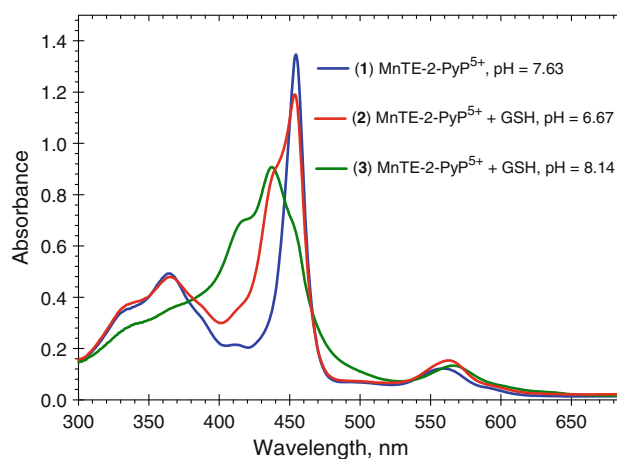
Fig. 7 The pH-dependent reduction of \text{MnTE-2-PyP}^{5+} with glutathione. Spectra were taken in 0.1 M tris buffer with 10 \mu\text{M} \text{MnTE-2-PyP}^{5+} and 0.7 mM glutathione. The pH values were: 7.63 (1), 6.67 (2), and 8.14 (3). Spectra were taken at 1 min after the reaction had started. The \text{Mn}^{\text{III}}\text{TE-2-PyP}^{5+} has the absorbance at 454 nm (spectrum 1) (Batinic-Haberle et al. 2002) and the reduced porphyrin \text{Mn}^{\text{II}}\text{TE-2-PyP}^{4+} at 438.4 nm (spectrum 3) (Spasojevic et al. 2000). The appearance of the shoulder at \sim 415 nm of the metal-free ligand (Batinic-Haberle et al. 2002) in spectrum 3 suggests that upon reduction a loss of Mn occurs to some extent. At higher pH > 9 , GSH is predominantly in a form of more reactive thiolate species in solution. The reaction of MnP with GSH at higher pH may resemble the in vivo conditions where protein cysteines have presumably lower pK_a values (Hill et al. 2009)
