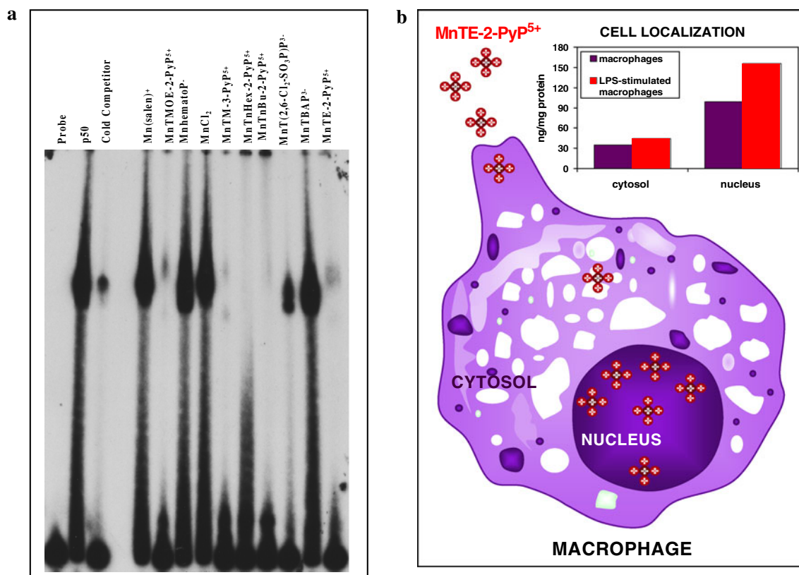
Fig. 8 a The electrophoretic mobility shift assay (EMSA) of NF-κB in the presence of several different anionic and cationic Mn porphyrins, Mn(salen) + (EUK-8) and MnCl 2 . The procedure was done as previously described (Tse et al. 2004). In brief, EMSAs with recombinant human NF-κB p50 (Promega) were performed in a cell-free system with the addition of anionic and cationic Mn porphyrins directly in the binding reaction for 15 min prior to the addition of 32 P-labeled NF-κB consensus oligo. The following final concentrations of Mn porphyrins were added to the binding reaction: 13.5 μM Mn(salen) + , 11 μM MnTMOE-2-PyP 5+ , 21.3 μM MnhematoP - , 10 μM MnCl 2 , 9.7 μM MnTM-3-PyP 5+ , 11.7 μM MnTnHex-2-PyP 5+ , 11 μM MnTnBu-2-PyP 5+ , 7.6 μM MnT(2,6-Cl 2 -SO 3 P) 3- ,
