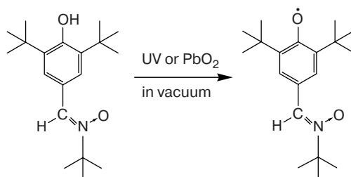
Fig. 1. Oxidation scheme of \alpha -(3,5-di- tert -butyl-4-hydroxyphenyl)- N - tert -butylnitron.
