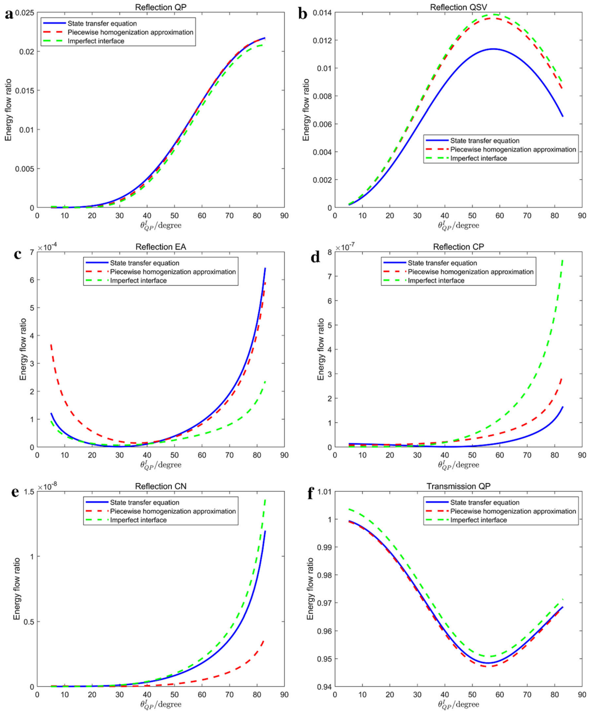
Fig. 6 The energy flux ratio of the reflection and the transmission waves with respect to incident wave for PN heterojunction. a RQP; b RQSV; c REA; d RCP; e RCN; f TQP; g TQSV; h TEA; i TCP; j TCN
