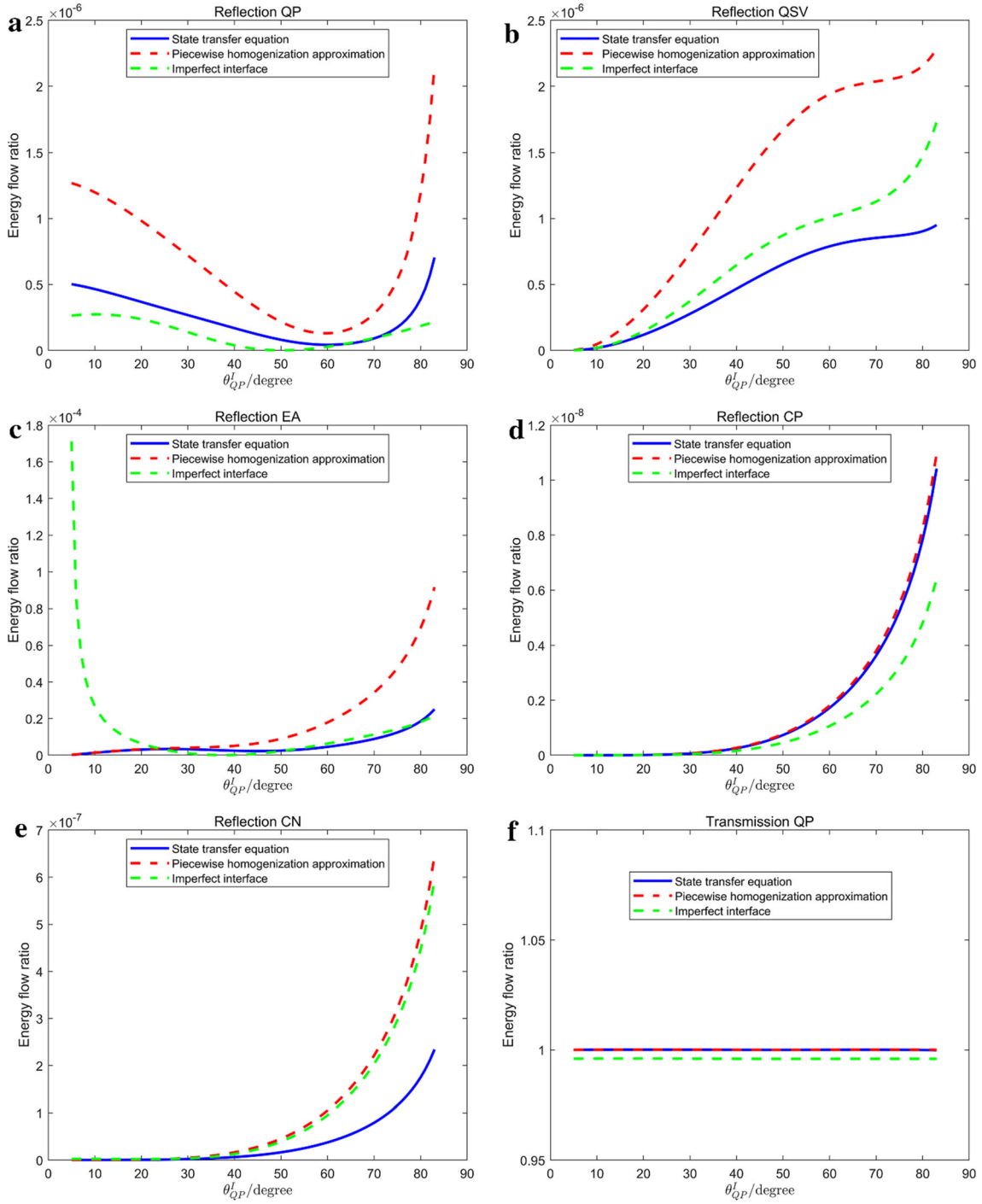
Fig. 4 The energy flux ratios of the reflection and transmission waves in the case of PN homojunction. a RQP; b RQSV; c REA; d RCP; e RCN; f TQP; g TQSV; h TEA; i TCP; j TCN
