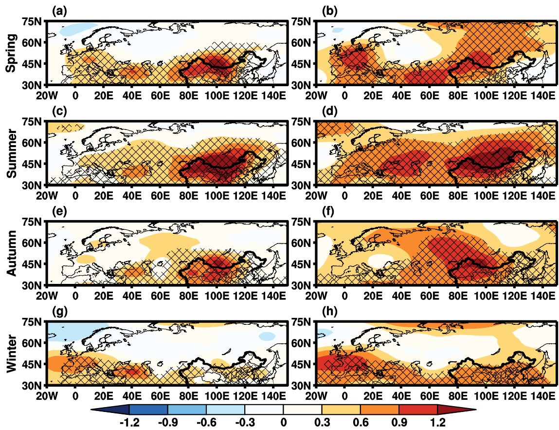
Fig. 9 Linear trend (unit, hPa decade -1 ) of seasonal mean geopotential height at 850 hPa (left panels) and 500 hPa (right panels) during 1960–2011. Hatching denotes the regions with statistical significance at 95% confidence level
