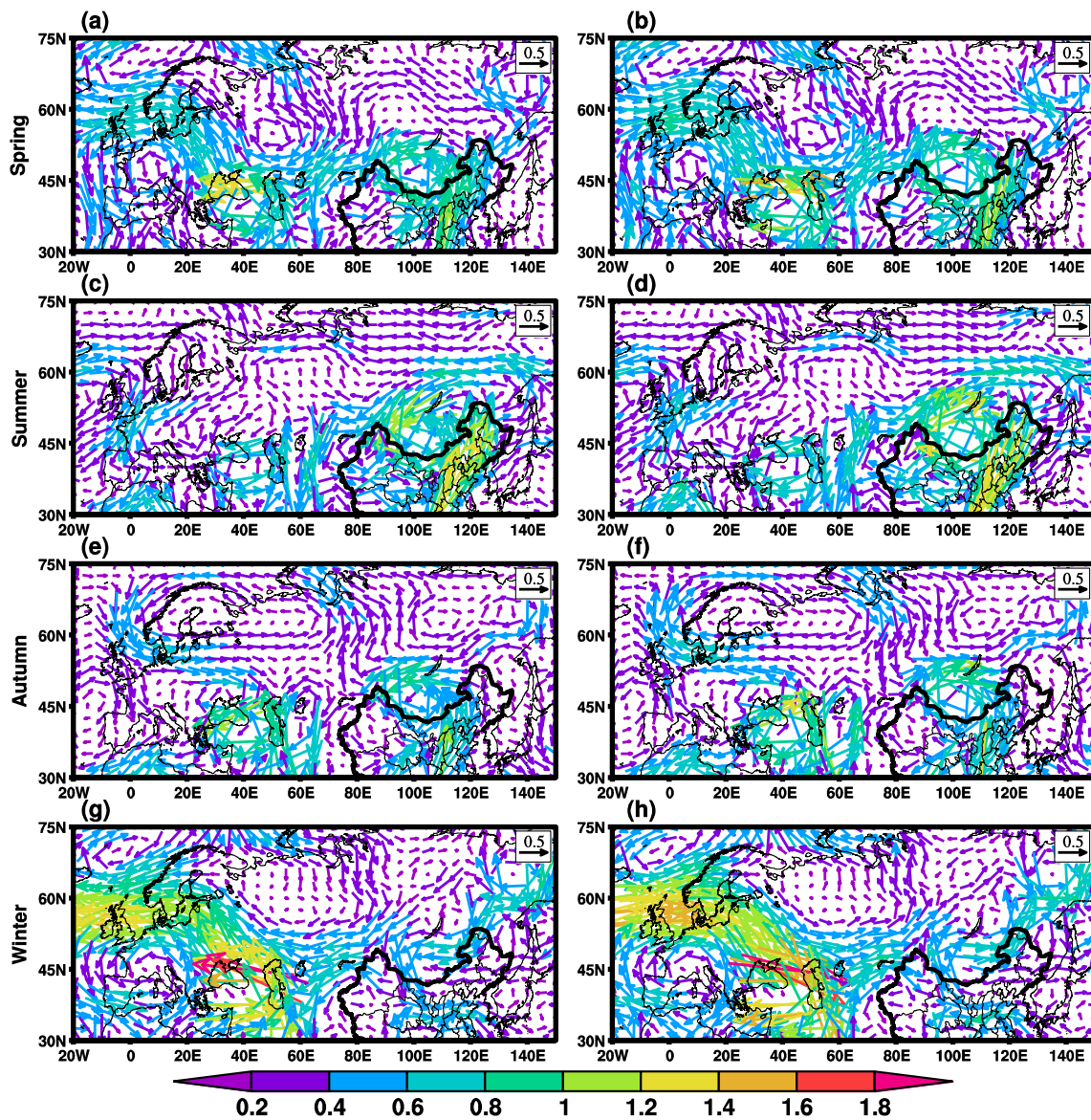
Fig. 8 Horizontal wind anomaly (unit, \text{m s}^{-1} ) between 1960–1986 and 1960–2011 (left panels), and between 1987–2011 and 1960–2011 (right panels) at 850 hPa
