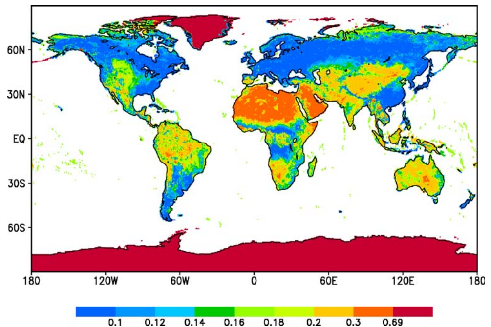
Fig. 2 Global distribution of soil albedo at 0.5° resolution
