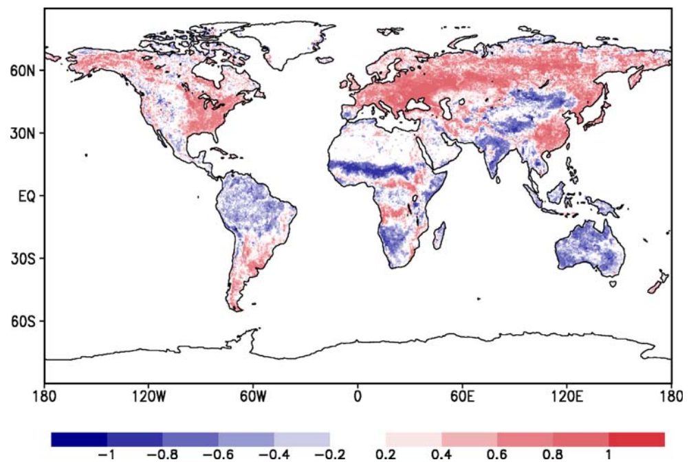
Fig. 1 Correlation between FPAR and albedo data from MODIS/Terra 2001–2004
