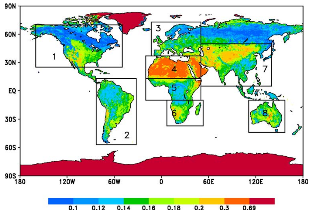
Fig. 4 Resulting annual mean of global background surface albedo climatology at 0.5° horizontal resolution for the climate models. The selected world regions are numbered for: 1 northern America, 2 southern America, 3 Europe, 4 northern Africa, 5 central Africa, 6 southern Africa, 7 southern Asia, 8 Australia
