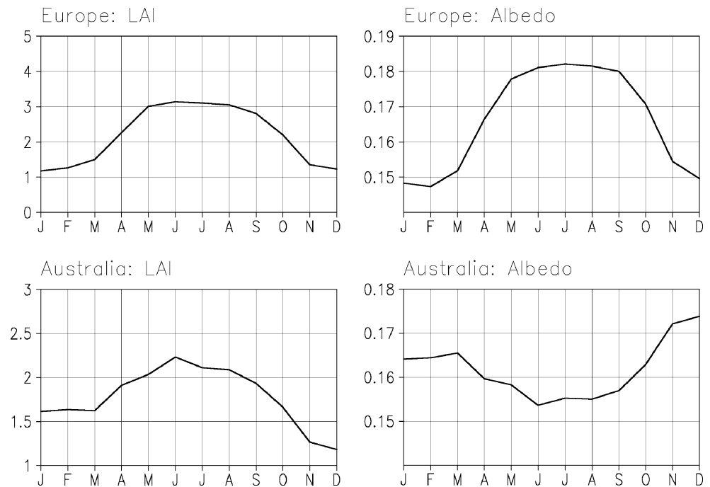
Fig. 6 Mean annual cycles of background albedo and LAI climatologies for Europe and Australia
