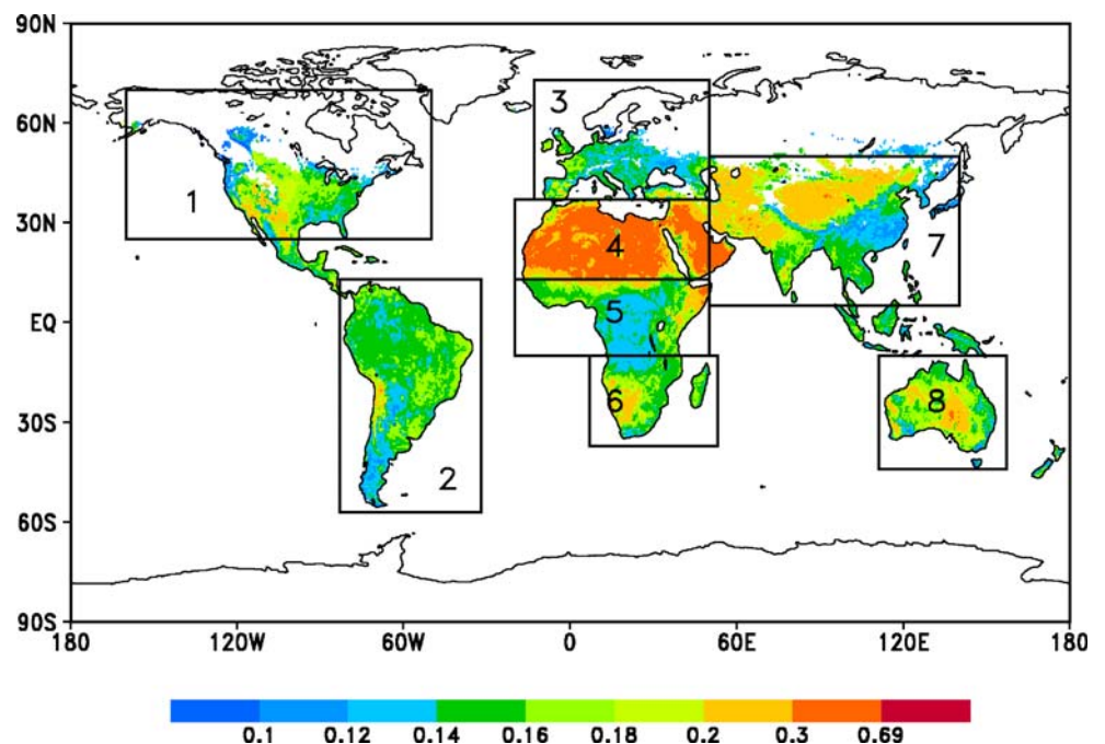
Fig. 5 Annual mean of global snow-free land surface albedo at 0.5° horizontal resolution of MODIS averaged over the whole period 2001–2004. The selected world regions are numbered as in Fig. 4. Values are only plotted at grid points, where MODIS is available for all months of the year
