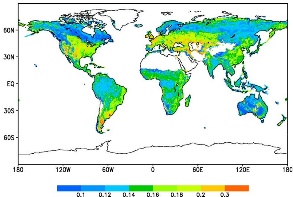
Fig. 3 Global distribution of vegetation albedo at 0.5° resolution
