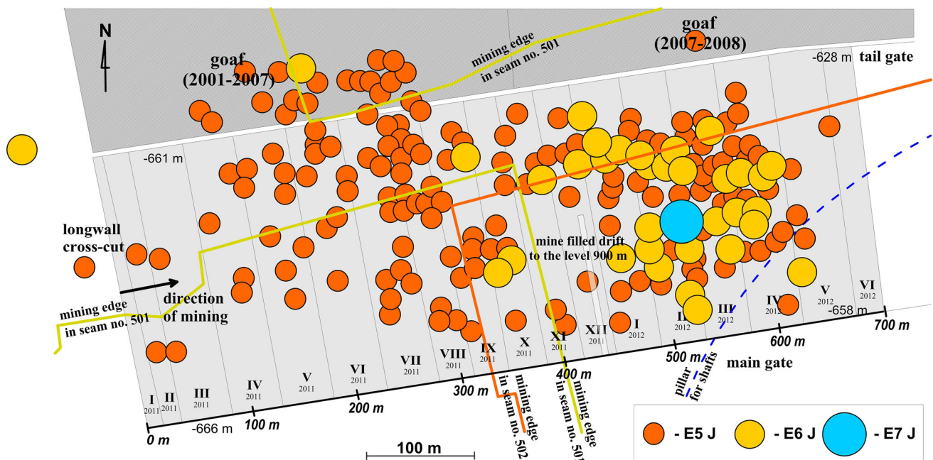
Fig. 2 Location of high-energy tremor sources induced during the longwall mining of coal seam no. 507 with the selected longwall (modified after Wojtecki and Koniecz 2016)
