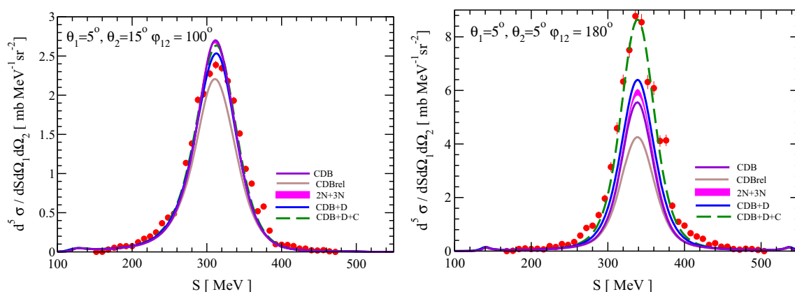
Fig. 2 Examples of the preliminary differential cross section of breakup reaction obtained for chosen kinematical configurations as a function of the S value at 340 MeV beam energy, red dots . Magenta band represents calculations based on realistic potentials: 2N complemented with the TM99 3NF and the realistic AV18 potential combined with the Urbana IX. The calculations within the coupled-channel approach with the CD Bonn + \Delta potential without (CDB + D) and with (CDB + D + C) the Coulomb force included are represented by blue solid line and green dashed line , respectively. Violet and brown solid lines present theoretical calculations with CD Bonn potential in nonrelativistic (CDB) and relativistic (CDBrel) regime, respectively (color figure online)
