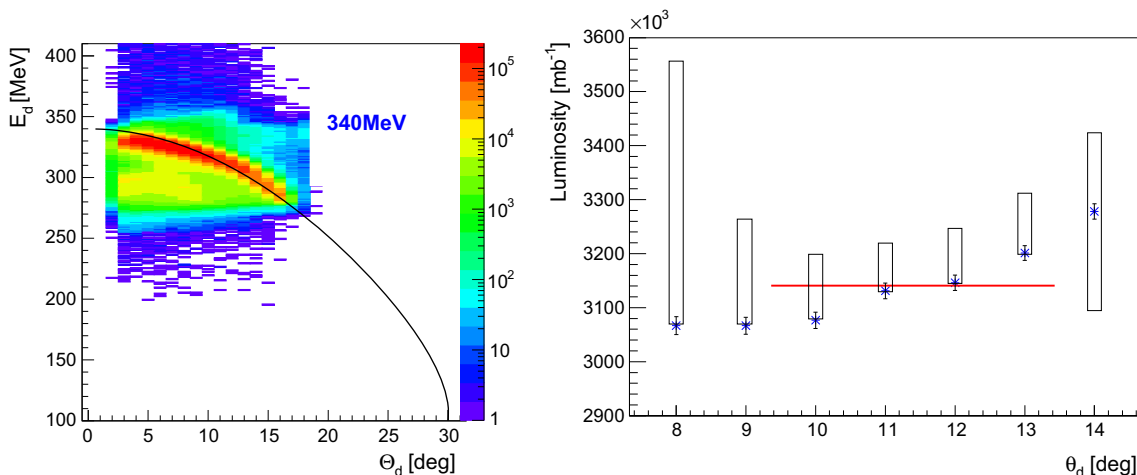
Fig. 1 Preliminary determination of luminosity. Left panel selection of deuterons registered in FD. Solid curve corresponds to kinematics for elastically scattered deuterons. Right panel the values of the luminosity presented as function of the deuteron scattering polar angle. The solid line corresponds to the weighted average of four results with the smallest systematic errors (shown as boxes). The error bars represent statistical uncertainties only
