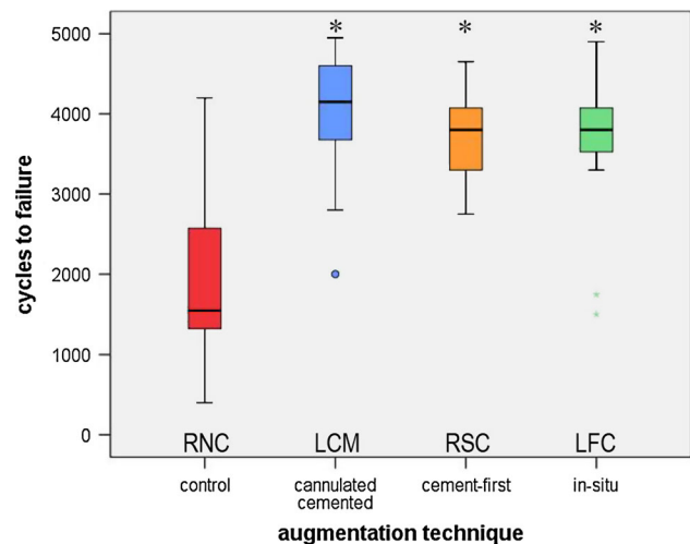
Fig. 4 The control screwing technique exhibited significant lower load cycles to failure compared to all other groups. The boxplots are showing the median, the 25th and the 75th quartile of the load cycles to failure for the four groups. Statistical significant differences to the control group are marked with an asterisk
