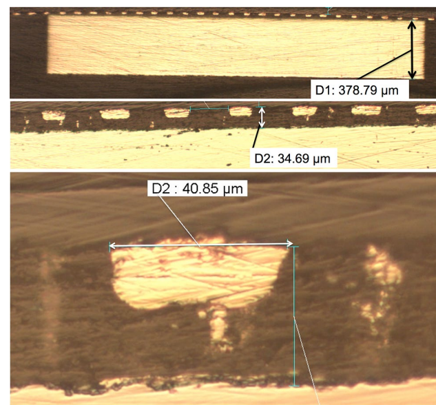
Fig. 14 Cross-section magnifications of a silicon electrical test die bonded to a FPCB at different scales, with different aligned conductive pillars visible at different depths. Note that an FPCB with a higher number of tracks (34 instead of 18) was used, but only 18 tracks are aligned to the die
