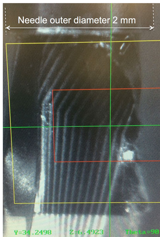
Fig. 10 Detail of the bonding site of the FPCB fed through the needle bore. The outer diameter of the needle is 2 mm
