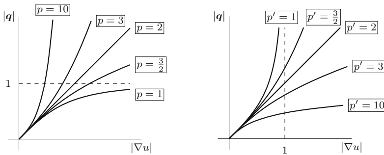
Fig. 2 On the left, the graphs of \mathbf{q} = (1 + |\nabla u|^2)^{\frac{p-2}{2}} \nabla u are sketched for selected values of p \in [1, \infty) , namely p = 1, \frac{3}{2}, 2, 3, 10 . On the right, the graphs of \nabla u = (1 + |\mathbf{q}|^2)^{\frac{p'-2}{2}} \mathbf{q} are shown for p' = 1, \frac{3}{2}, 2, 3, 10 .
