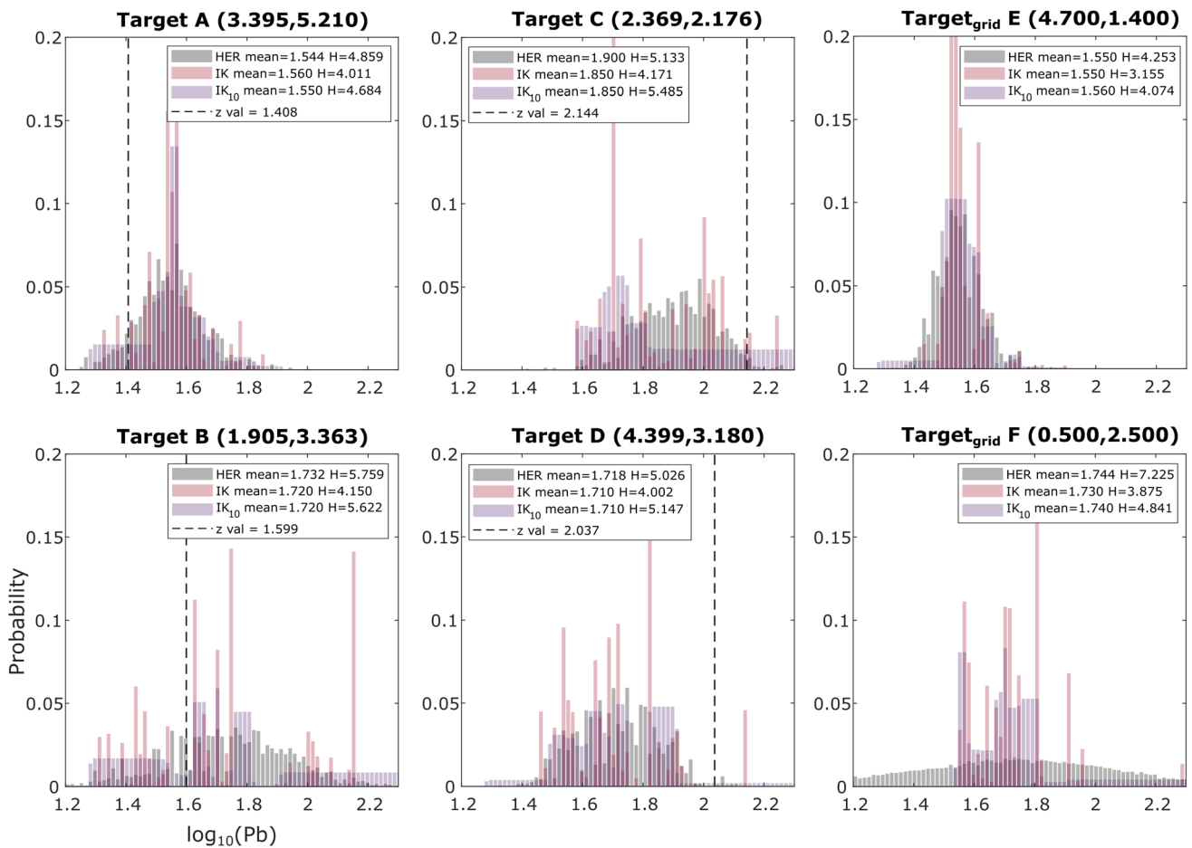
Fig. 18 Local distribution of targets of the validation set (targets A to D) and grid (targets E and F) for HER (gray), IK (red), and \text{IK}_{10} (purple)
