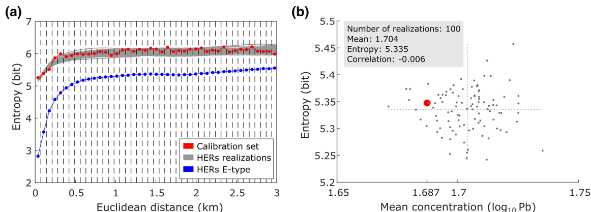
Fig. 11 Ergodic fluctuations of 100 realizations generated with HERs. a Infogram and b scatterplot of the mean and entropy values
