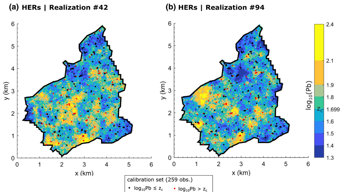
Fig. 12 Realizations generated using HERs. a Realization #42 and b realization #94. Simulation grid size of 0.05 km × 0.05 km
