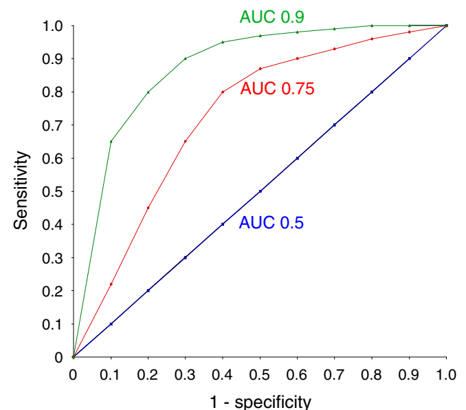
Fig. 1 Three hypothetical receiver-operating characteristic (ROC) curves are shown. The blue (straight) line represents a biomarker with an area under the curve (AUC) of 0.5, which indicates a result that is no better than expected by random chance. The red (middle) curve yields an AUC of about 0.75, which is generally considered a good biomarker. The green (top) curve gives an AUC of approximately 0.9, which would represent an excellent biomarker
