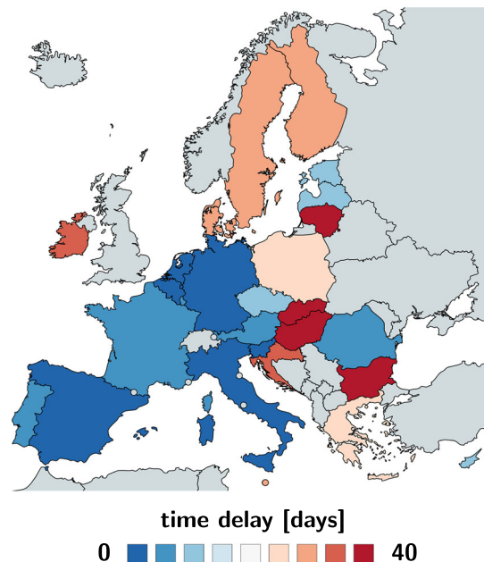
Fig. 7 Time delay \Delta t between reduction of air travel and reduction of the effective reproduction number across Europe. The time delay characterizes the mean time between the reduction in air travel, driving, walking, and transit mobility and the reduction in the effective reproduction number. It has maximum values in Bulgaria and Slovakia with 43.00 and 40.25 days and minimum values in Germany and the Netherlands both with 3.25 and 0.75 days
