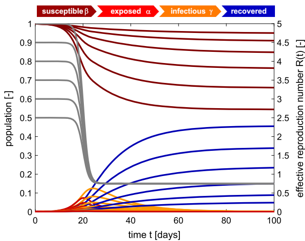
Fig. 8 SEIR model with time-varying effective reproduction number. Increasing the basic reproduction number R_0 increases the initial growth, and with it the number of cases. The temporary equilibrium for the smaller basic reproduction number of R_0 = 2.5 is s_\infty^* = 0.948 and r_\infty^* = 0.052 and for the larger basic reproduction number of R_0 = 5.0 is s_\infty^* = 0.544 and r_\infty^* = 0.456 . Latent period A = 2.5 days, infectious period C = 6.5 days, basic reproduction number R_0 = [5.0, 4.5, 4.0, 3.5, 3.0, 2.5] , effective reproduction number R_t = 0.75 , adaptation time t^* = 20 days, and transition time T = 15 days
