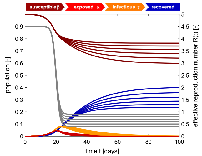
Fig. 9 SEIR model with time-varying effective reproduction number. Increasing the reproduction number R_t decreases the effect of interventions and increases the number of cases. The temporary equilibrium for the smaller effective reproduction number of R_t = 0.4 is s_\infty^* = 0.764 and r_\infty^* = 0.236 and for the larger effective reproduction number of R_t = 0.9 is s_\infty^* = 0.594 and r_\infty^* = 0.406 . Latent period A = 2.5 days, infectious period C = 6.5 days, basic reproduction number R_0 = 4.5 , effective reproduction number R_t = [0.4, 0.5, 0.6, 0.7, 0.8, 0.9] , adaptation time t^* = 20 days, and transition time T = 15 days
